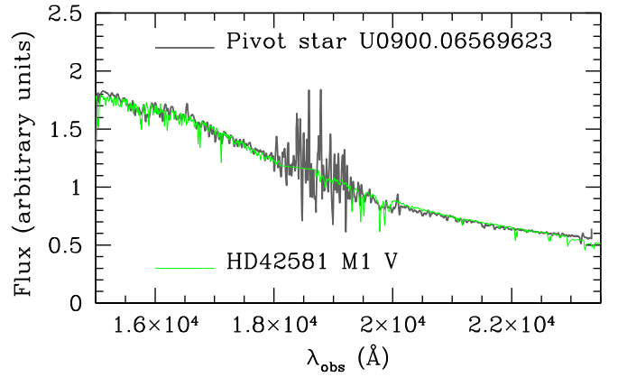
Figure 1. Final LBT-LUCI 1D spectrum of the pivot star U0900.06569623 smoothed over 4 pixels ( \sim 17 Å; gray curve) compared with the spectrum of the main-sequence M-type star HD 42581 (green curve). The two spectra have been normalized to the mean flux measured in the wavelength range 1.7 – 1.8 \mu\text{m} . The comparison shows the perfect recovery of the true shape of the spectrum thanks to the careful correction for the response function of the instrument.
