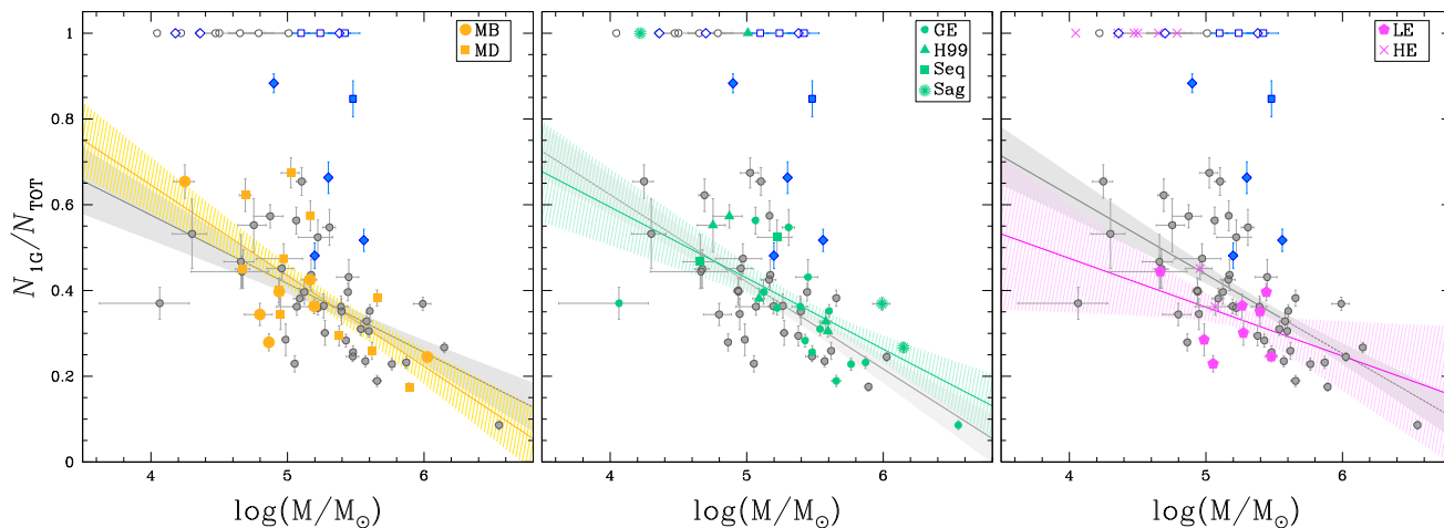
Figure 12. Each panel is a reproduction of the upper-left panel of Fig. 7 where we plot the fraction of 1G stars against the present-day mass of the host GC. The blue colours indicate LMC (squares) and SMC clusters (diamonds). Simple- and multiple-population GCs are indicated with open and filled symbols, respectively. In the left-hand, middle, and right-hand panels, we used yellow, aqua, and magenta colours to plot Milky Way GCs formed in situ , GCs that are the results of mergers, and other GCs with either high or low energy, respectively. The different coloured symbols indicate the progenitor structure according to Massari et al. (2019). GCs not in the specific categories are plotted as grey symbols. The corresponding least-square best-fitting lines are represented with the same colours and the shaded areas include the 68.27 per cent confidence interval of the true regression.
