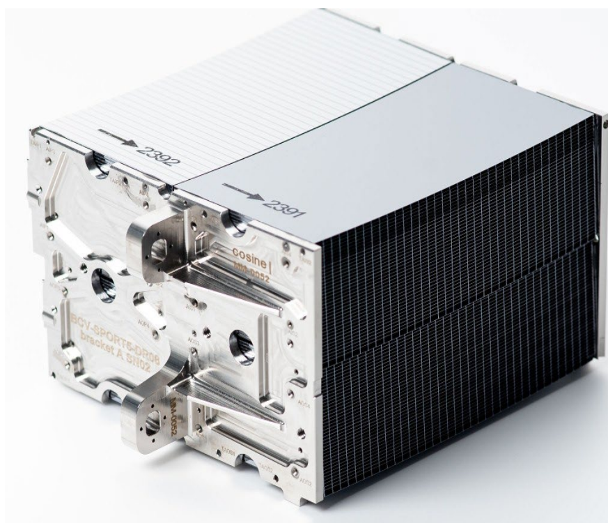
Figure 5: The NewATHENA optics consists of 492 SPO mirror modules, concentrically arranged in 13 rows; the figure shows a mirror module for the eighth row. The production processes used in the current development phase are largely the same as will be used for the flight implementation phase, ensuring a smooth transition between the phases. The actual mirror plates are only paper thin, 150 \mu\text{m} , and are fabricated with automated equipment spun-in from the semiconductor industry, starting with 300 mm diameter, 0.775 mm thick latest generation Silicon wafers. Each mirror module consists of four stacks of mirror plates, carefully aligned using synchrotron radiation to produce a single focus. The four stacking robots required to produce the mirror stacks for the flight implementation phase (about 2500 including spares etc) already exist.
