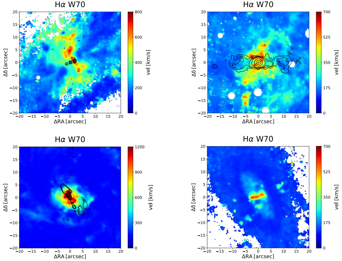
Fig. A.1: H\alpha W70 of IC 5063, NGC 5643, NGC 1068, and NGC 1386 (from top left to bottom right). The radio contours are superimposed (see main text for more details on reported radio data). The maps are zoomed in the central 40'' \times 40'' as in the [O\text{ III}] W70 maps of each respective galaxy (Figs. 2b, 5b, 7b, and 10b).
