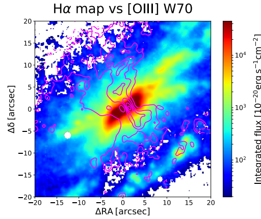
Fig. A.2: Map of H\alpha emission of IC 5063. The [O\text{ III}] W70 contours are superimposed. The map shows that the stripe of H\alpha star-forming (as indicated by the BPT diagram in Fig. 2c,d) clumps to the SW of the nucleus are in the direction of the high-W70 material, approximately at its edge.
