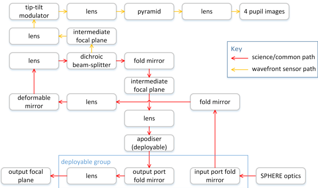
Figure 1. Optical block diagram of SAXO+. The starting block is “SPHERE optics” at the bottom-right. With this choice, somehow unconventional, the order of the blocks in this conceptual diagram approximately reflects the order of the elements in the optical model shown in Fig. 2 and in the mechanical models shown later in the paper.
