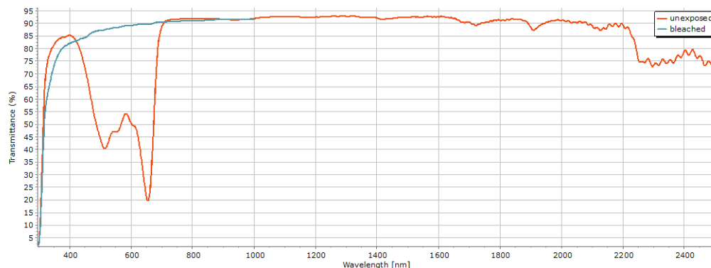
Figure 5. Transmission spectrum (no correction of the reflection losses) for a panchromatic Bayfol®HX film (17 μm thick) on TAC substrate before and after bleaching.
