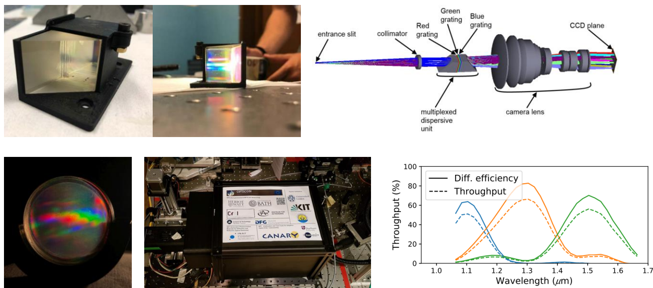
Figure 13. On top: photos of the three layers visible GRISM and the optical scheme. On the bottom: the three layers VPHG for MCIFU, the instrument on the optical bench of CANARY and the diffraction efficiencies of the three layers.
