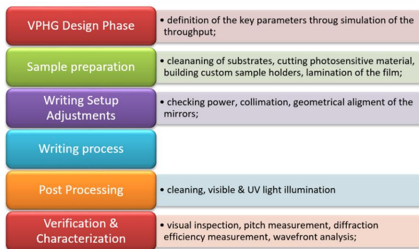
Figure 6. Scheme of the production steps developed for the production of Bayfol®HX based VPHGs.
