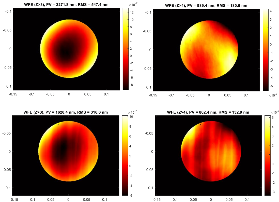
Figure 10. On top: Phase maps for the Red (top) and Blue (bottom) VPHGs. On the left the Zernike terms > 3 are considered; on the right the terms > 4 (the focus term is removed).
