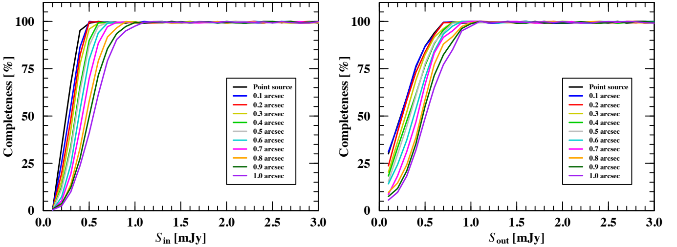
Fig. 8. Completeness as a function of the input flux density ( S_{in} ; left panel) and as a function of the output flux density ( S_{out} ; right panel) for different model source sizes ranging from pure point sources to 1'' FWHM.
