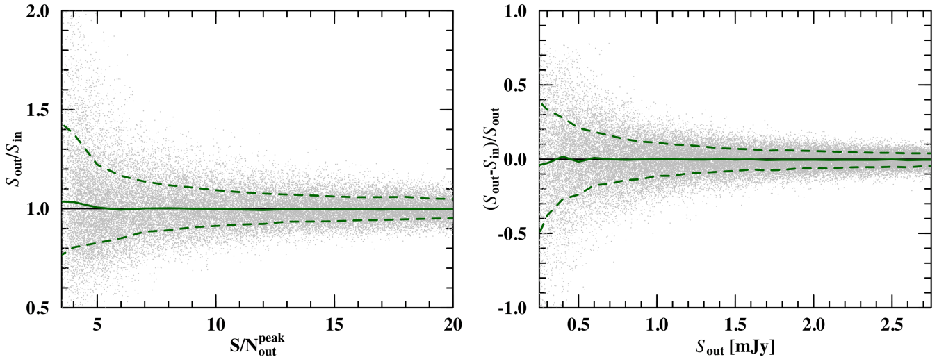
Fig. 9. Ratio of the output over input flux densities ( S_{out}/S_{in} ) as a function of the output detection S/N_{out}^{peak} ( S/N_{out}^{peak} ) from PyBDSF, measured as the peak flux density over the local rms noise (left panel), and flux density accuracy ( (S_{out} - S_{in})/S_{out} ) as a function of the output flux density ( S_{out} ) measured with the aperture photometry methodology (right panel) for simulated sources with sizes ranging 0''.1-0''.4 FWHM. The distribution of the whole set of simulations is shown as gray symbols with their sliding median and standard deviation in solid and dashed green, respectively.
