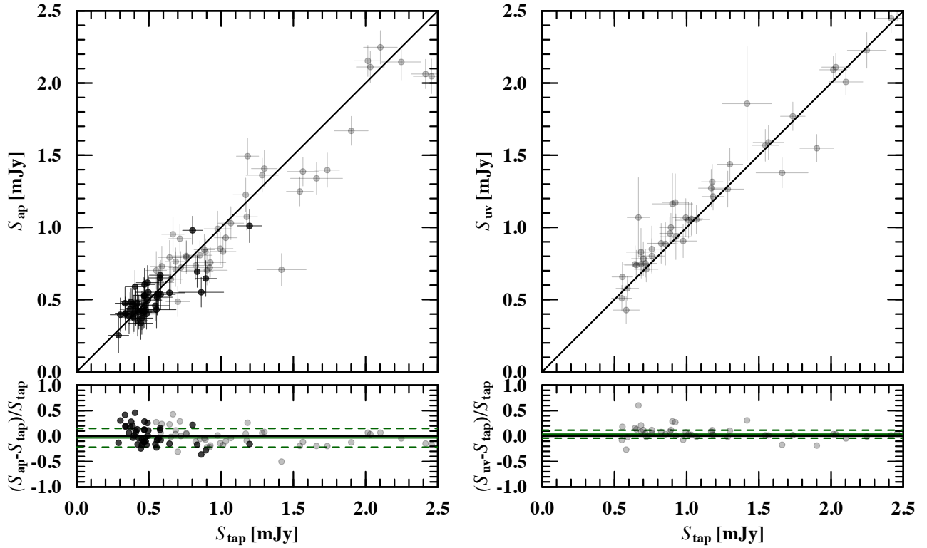
Fig. 7. Left panel: comparison between the flux densities obtained using the aperture and the tapering methodologies for both the 100% pure main catalog (gray symbols) and the prior-based supplementary catalog (black symbols). The median relative difference is (S_{\text{ap}} - S_{\text{tap}})/S_{\text{tap}} = -0.03 \pm 0.18 (shown with green lines in the bottom panel ). Right panel: comparison between the flux densities associated to the size measurements in the uv plane and the flux densities from the tapering methodology for the 100% pure main catalog (gray symbols). The median relative difference in this case is (S_{\text{uv}} - S_{\text{tap}})/S_{\text{tap}} = 0.04 \pm 0.08 .
