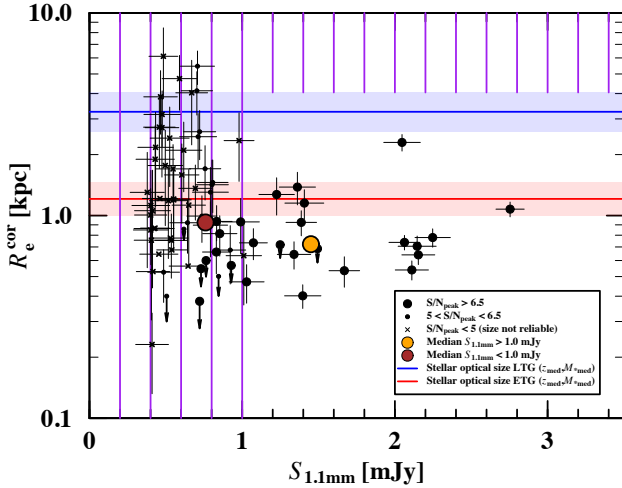
Fig. 16. Physical dust continuum size at 1.1 mm corrected to a common redshift and stellar mass ( z_{med} = 2.46 and \log(M_{*med}/M_{\odot}) = 10.79 ) versus 1.1 mm flux density for the sources in the 100% pure plus prior-based catalogs from the combined dataset. For sources in the 100% pure main catalog we distinguish detection S/N_{peak} > 6.5 (big black circles, representing approximately the top third of the source catalog) and detection 5 < S/N_{peak} < 6.5 (small black circles). The sizes of sources in the prior-based supplementary catalog (which have a detection S/N_{peak} < 5 ) are unreliable (shown as crosses), but their 1.1 mm flux densities are well constrained and, thus, we know their position in the x-axis. Median corrected dust continuum sizes for S_{1.1mm} > 1 mJy sources (orange circle) and S_{1.1mm} < 1 mJy sources (brown circle) are also displayed. The typical size of the stellar distribution measured at optical wavelengths for both early and late-type galaxies from van der Wel et al. (2014) at z_{med} and M_{*med} are also shown with their scatter as a shaded areas. The grid of purple lines shows the region where we are no longer \sim 100\% complete. Compact dust continuum emission at S_{1.1mm} > 1 mJy prevails and sizes as extended as typical star-forming stellar disks in this flux density regime are rare.
