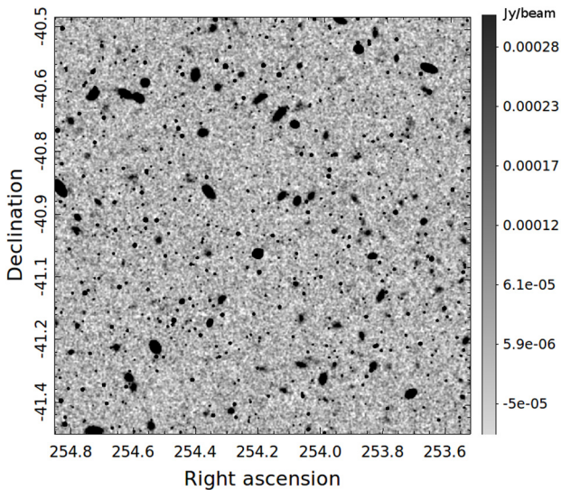
Fig. 6. A sample simulated map ( 900 \times 900 pixels, 1 \text{ deg}^2 area) produced for the testing campaign. FWHM synthesized beam is equal to 15'' and Gaussian noise has a 20 \mu\text{Jy}/\text{beam} rms. Point sources were injected uniformly spaced and with flux density S following \exp^{-\lambda S} ( \lambda = 1.6 ) and ranging from 50 \mu\text{Jy} to 1 \text{ Jy} . Extended sources were injected uniformly spaced from a 2D elliptical Gaussian model with randomized axes, up to a maximum major axis size of 3 \times beam size and minor/major axis size ratio varying from 0.4 to 1. Flux densities S were generated according to \exp^{-\lambda S} ( \lambda = 1.6 ) and ranging from 5 \mu\text{Jy} to 1 \text{ mJy} . Total source density is equal to 2500 \text{ deg}^{-2} , with a fraction of 10% of extended sources.
