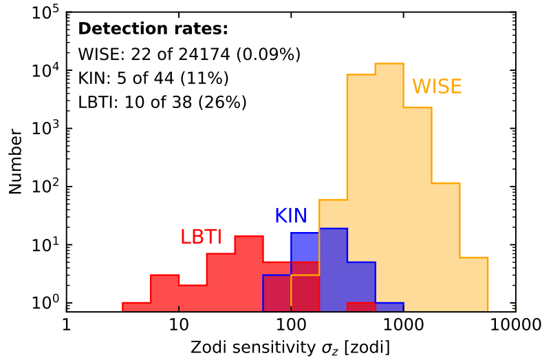
Figure 3. Distribution of sensitivity to habtable zone dust and sample sizes of LBTI, 25 KIN, 26 and WISE. 27 The unit of 1 zodi corresponds to the habitable zone dust surface density in the Solar system.
