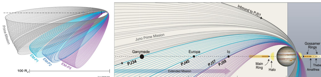
Figure 1. Left panel. The Juno orbit petal has been evolving due to the oblateness of Jupiter, such that perijove is moving north and apojove is moving south. The prime mission orbit period was 53 days; in the extended mission the orbital period has decreased to 43 days (phase P1), will shrink to 38 days after the close Europa flyby (P2) and finally to 33 days (P3) due to the effect of the moons' gravity on the close flybys. Right panel. In 2021 the inbound leg of Juno's orbit crossed the orbit of Ganymede, with the opportunity to observe Ganymede at an altitude of 1,046 km prior to P34, and at an altitude of approximately 50,000 km prior to P35.
