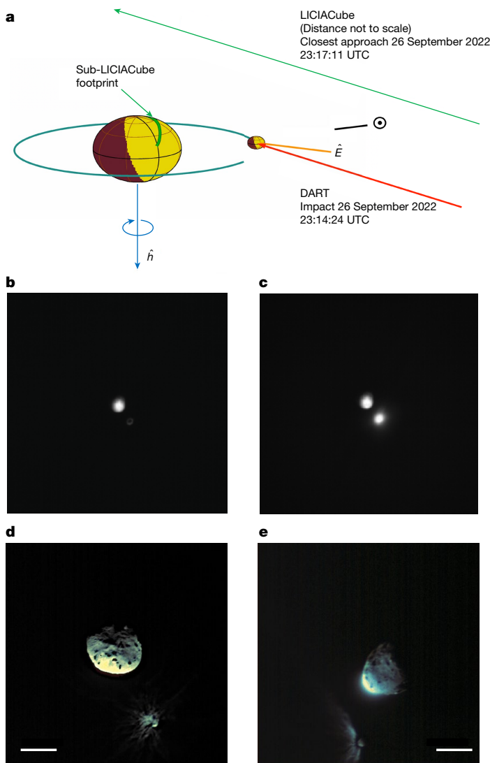
Fig. 1 | The viewing geometry of LICIACube. a–e. Schematic of the DART impact and LICIACube viewing geometries (a) and cropped images of Didymos and Dimorphos as seen by LEIA (b,c) and LUKÉ (d,e). a, The trajectory and the footprint on Didymos are shown in green; \hat{h} is the positive pole direction of Didymos; the red arrow is the incident direction of the DART; \hat{E} is the cone axis pointing; the relative direction of the Sun is also shown in yellow. b, The binary system imaged at a distance of approximately 1,000 km, 5 s before the impact: Didymos is visible in the centre of the LEIA FOV and Dimorphos appears as a ring (because of the de-focusing of the instrument, discovered on flight) at the lower right side of Didymos. c, The same scene viewed 1 s after the impact: the expanding ejecta plume causes an increase of a factor 5, in terms of DN over the same area in the lower right side of Didymos. d, RGB image of the targets acquired at a distance of 76 km, 8.5 s before CA (159 s after impact). e, RGB image at a distance of 71 km, 6.5 s after CA (174 s after impact). Scale bars, 500 m (d,e).
