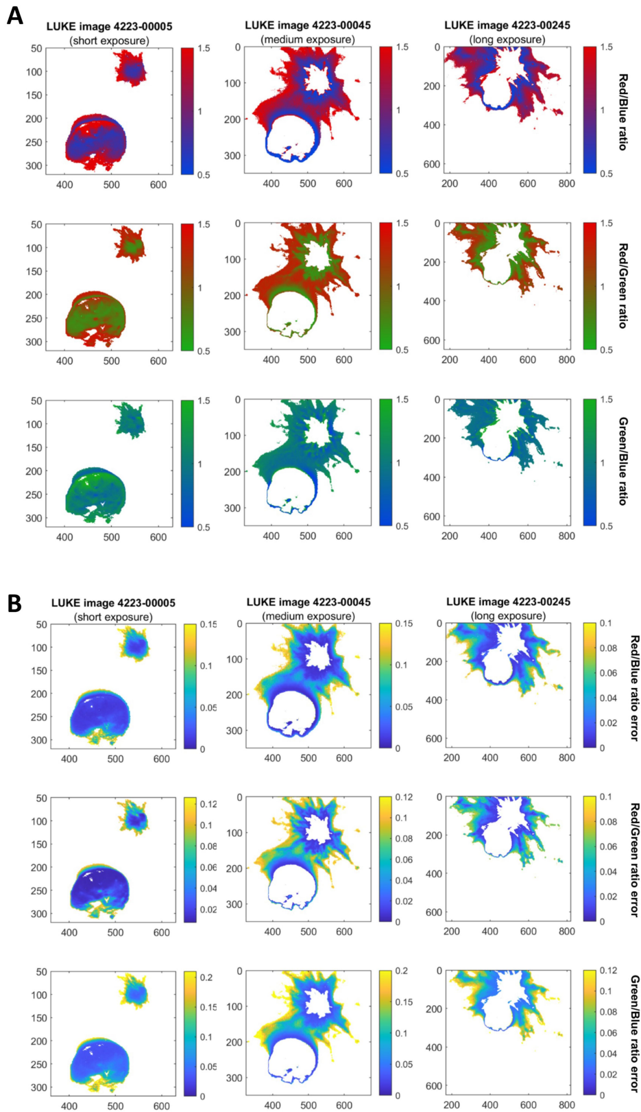
Extended Data Fig. 7 | Didymos-Dimorphos maps of flux ratio in LUKExposure colour filter data. Flux ratio (panel A, top) and fluxes ratio error (panel B, bottom) for LUKExposure images at different exposure times (see RGB analysis method text
