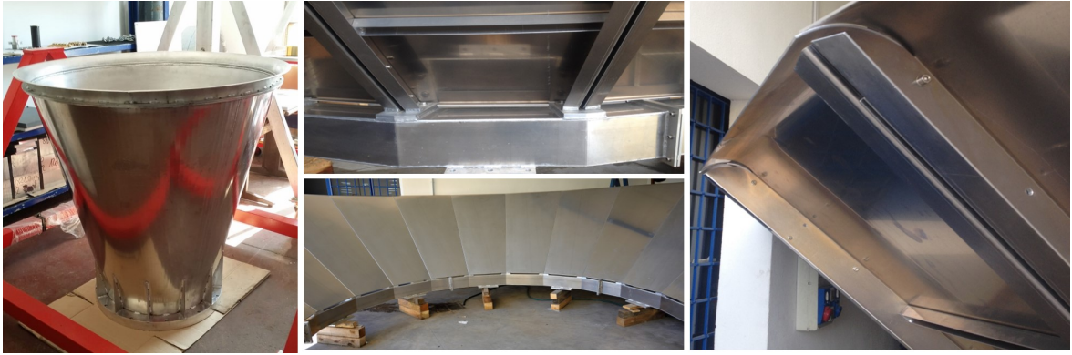
Figure 24. The FB during manufacturing (left) and details of the GS: base (top middle), inner panels (bottom middle) and flare (right).
