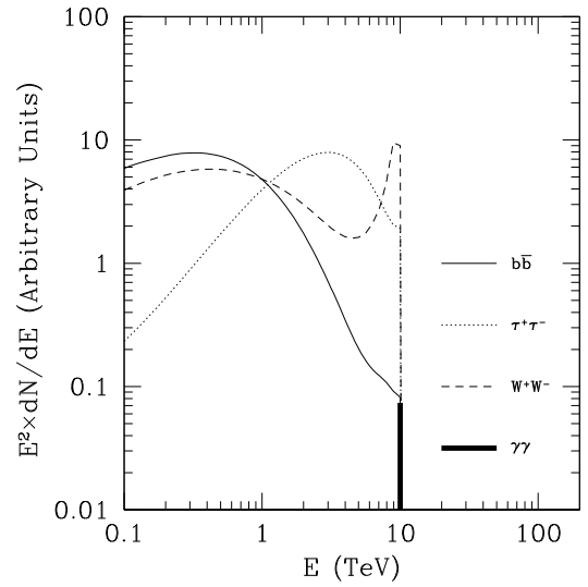
Fig. 9. Example spectra produced by DM annihilation for m_\chi = 10 TeV for the four SM channels considered: b\bar{b} (thin solid line), \tau^+\tau^- (dotted line), W^+W^- (dashed line) and \gamma\gamma (thick solid line).
