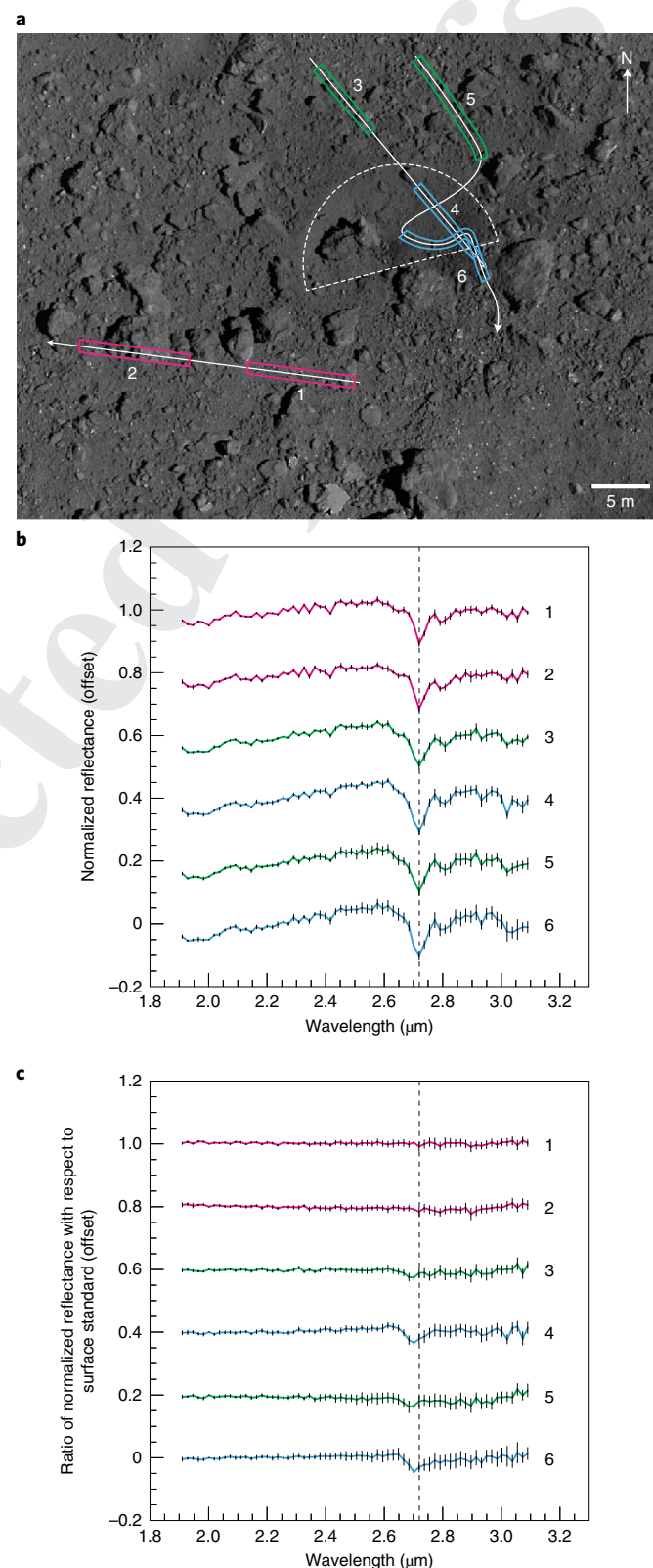
Fig. 1 | NIRS3 observations of the SCI crater region. a , Context image taken by the ONC-T camera. The dashed semi-circle represents the rim of the SCI crater 4 . The arrows indicate the motion of NIRS3 footprints during three descent operations. b , NIRS3 spectra averaged over regions corresponding to the coloured boxes shown in a . The colour of each site represents its surface characteristics: magenta, green and cyan are the ejecta-free region, ejecta-rich region outside the crater and ejecta-rich region inside the crater, respectively. Error bars are 1σ within the boxes. Individual spectra of each site are shown in Extended Data Fig. 1. c , Ratios of the normalized spectra shown in b to the ones of the surface standard observed on the day before. The spectra are normalized and vertically shifted for clarity. The dashed vertical lines at 2.72 μm denote the peak wavelength of the OH absorption of the spectra in b .
