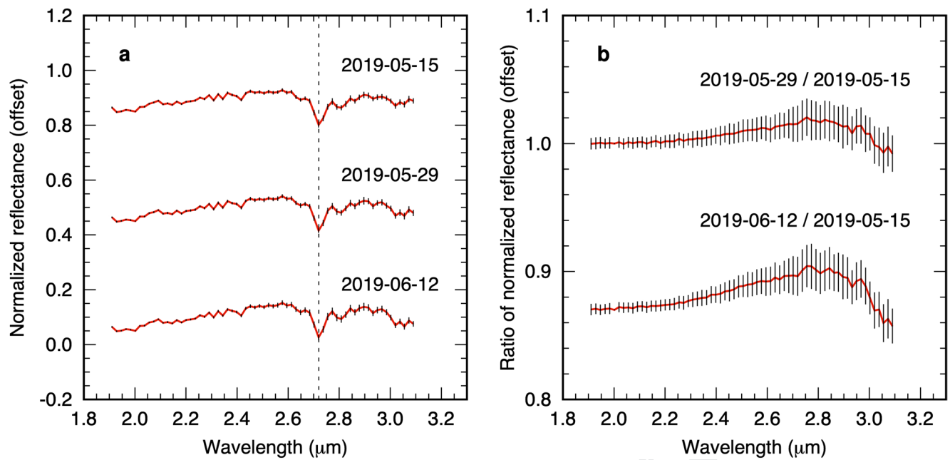
Extended Data Fig. 4 | NIR53 spectra of the surface standard. a , Spectra averaged over regions having the similar surface temperature to the SCI crater region. The details of these spectra are listed in Extended Data Fig. 3. b , Ratios between the normalized spectra shown in a . The non-flat shape of the ratio-spectra indicates the residual of thermal correction. The spectra are normalized and vertically shifted for clarity. Note that the vertical scale of b is much larger than that of a to show the curvature and uncertainties of the ratio-spectra.
