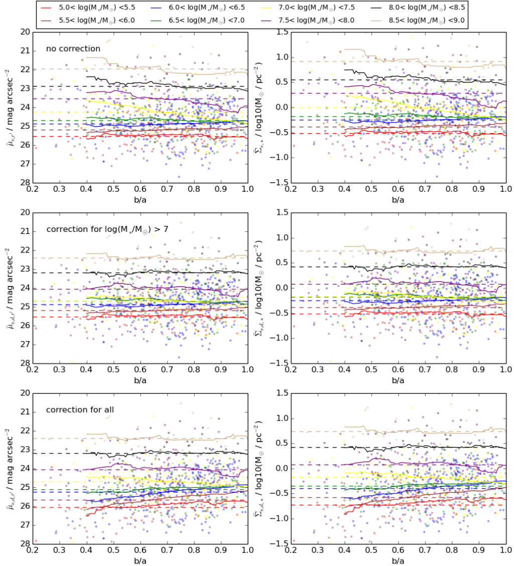
Fig. 11. Inclination corrections. Correlation between the axis ratio ( b/a ), mean effective SB ( \bar{\mu}_{e,r'} ), and stellar SD ( \bar{\Sigma}_{e,*} ) of the galaxies. Upper panels: values without any inclination corrections, in the middle panels galaxies with \log(M_*/M_\odot) > 7 have been corrected for their inclination, and in the bottom panels inclination correction has been applied to all the galaxies. The different colors correspond to different mass bins, as shown in the legend. The solid and dashed lines indicate the running mean (filter size of 0.2) and the mean of the mass bin.
