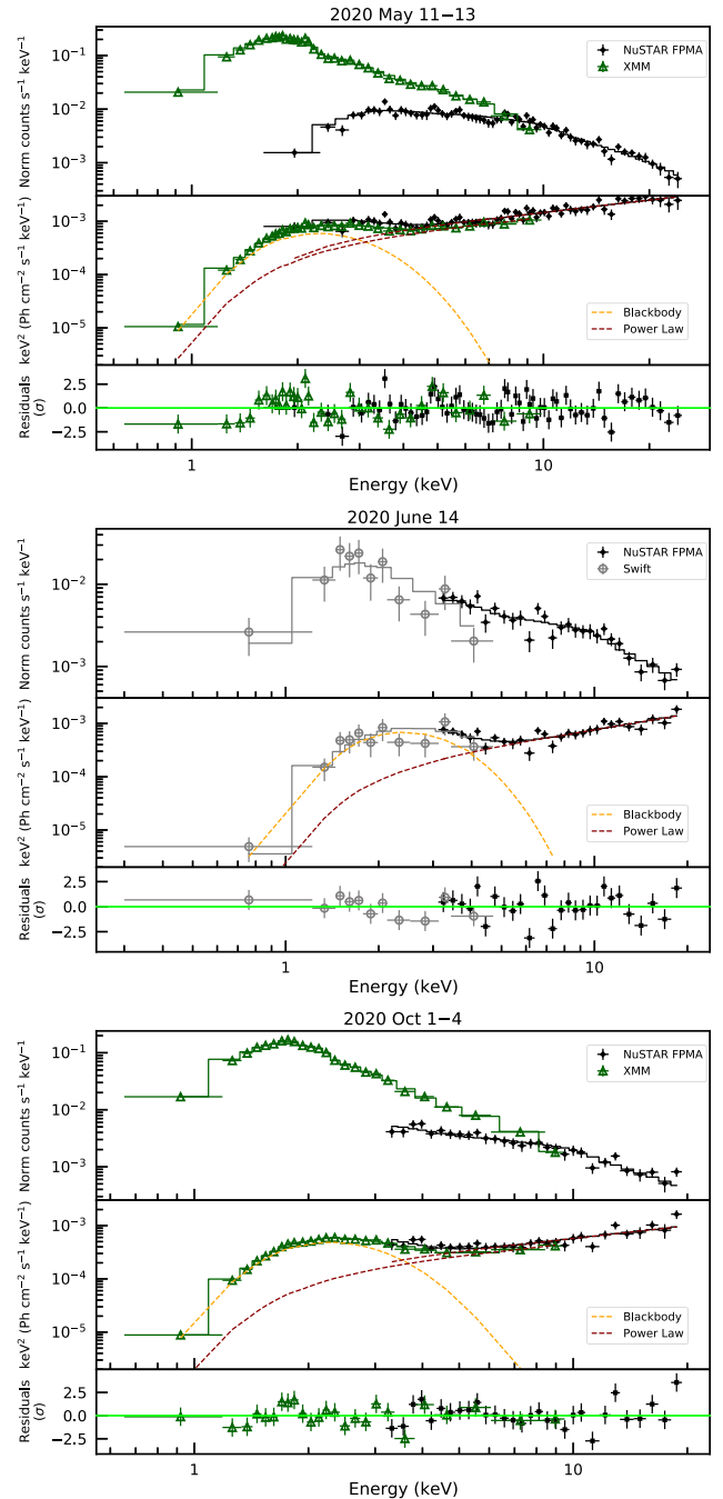
Figure 2. Broad-band spectra of SGR J1935 extracted from the quasi-simultaneous Swift /XRT (grey), NuSTAR (black), and XMM-Newton (green) data on 2020 May 11–13 (top), June 14 (middle), and October 1–4 (bottom). XMM-Newton data were re-binned for plotting purpose. For each plot, the E^2 f(E) unfolded spectrum is shown in the middle panel. The dashed lines mark the contribution of the single components to the spectral model. Post-fit residuals in units of standard deviations are shown in the bottom panel.
