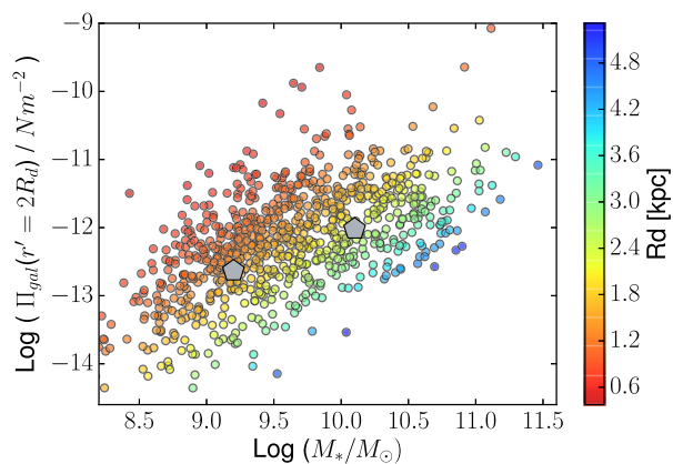
Figure 4. Replaces Fig. 5 in the original paper (almost identical). The anchoring force at r' = 2 \times R_d as a function of stellar mass for all spiral galaxies in our (cluster plus field) sample, colour-coded by R_d . The pentagons correspond to the model galaxies I and II.
