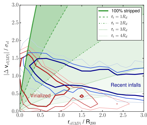
Figure 5. Replaces Fig. 6 of the original paper (green area broadened towards the right of the plot). Position versus velocity phase-space diagram of 15 simulated group and cluster galaxies (mass range from 0.5 \times 10^{13} to 1 \times 10^{15} M_\odot ) from Rhee et al. (2017, private communication); using the YZICS simulations by Choi & Yi (2017), considering multiple lines of sight, separated into ‘virialized’ (entered the cluster >4 Gyr ago; red contours) and ‘Recent infalls’ (falling towards the cluster for the first time or recently entered the cluster <2 Gyr; blue contours). A galaxy is considered to enter the cluster when it has crossed R_{200} for the first time. The contours enclose 1000, 2500, and 5000 particles from lighter to darker colours respectively. The axes have been normalized by cluster size ( R_{200} ) and cluster velocity dispersion ( \sigma_{cl} ) to allow the stacking of different clusters. The green area indicates the increasing effect of ram-pressure stripping by the ICM in the case of a low-mass galaxy (model galaxy I) falling in a massive cluster (model cluster B). The green lines correspond to different truncation radius ( r_t ) in units of stellar disk scale length ( R_d ). For details see Section 3, and Tables 1 and 2 of the original paper.
