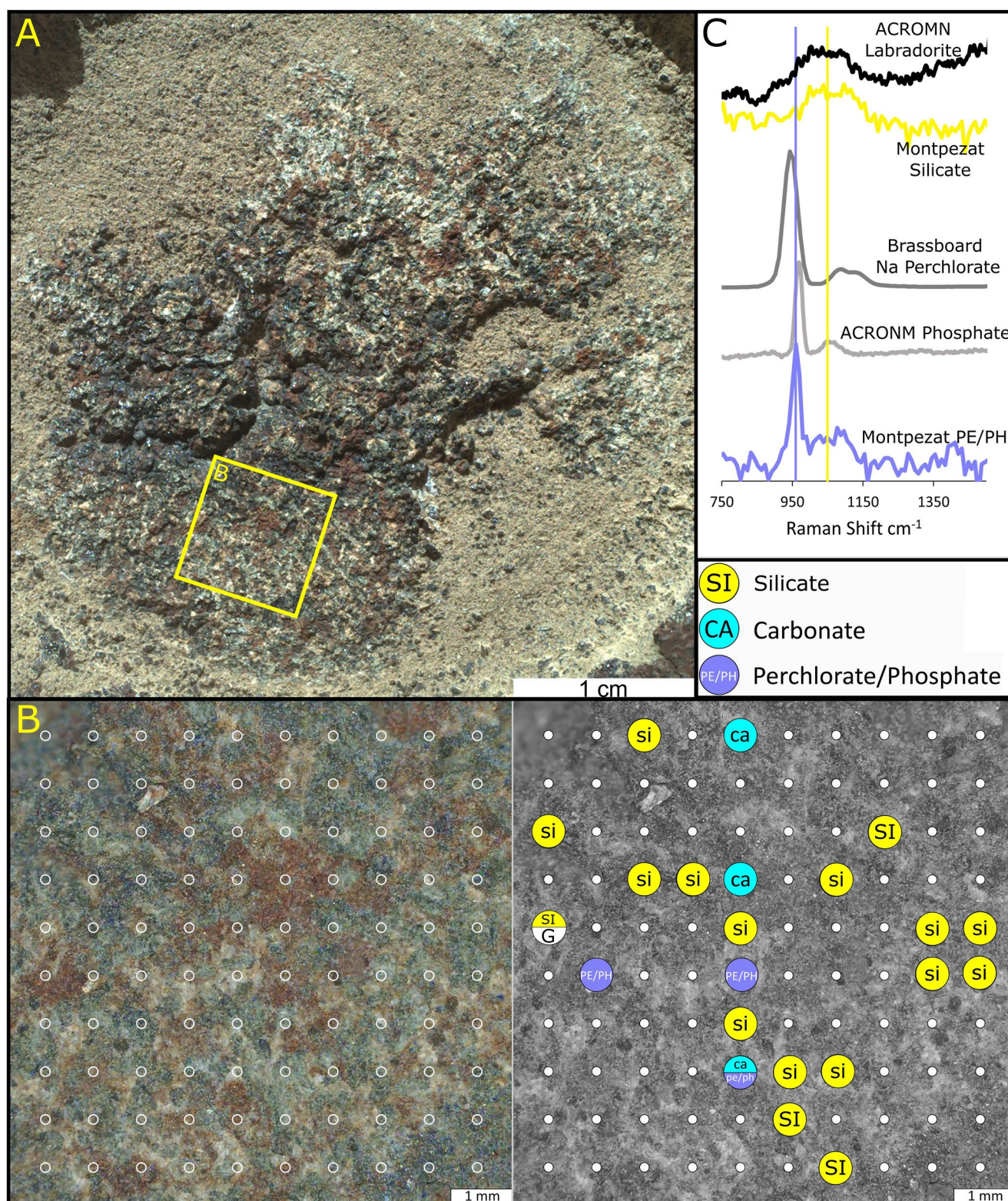
Figure 6. SHERLOC Raman mineral identifications from the 0349_Montpezat HDR_500_1 scan of the target Montpezat. (a) The abrasion patch imaged by WATSON (image ID SIF_0346_0697661461_972FDR_N0092982SRCL01034_0000LMJ01). The yellow box indicates the location of the scan. (b) Colorized (left) and grayscale (right) ACI images (image ID SC3_0349_0697954126_179FDR_N0092982SRCL10600_0000LMJ01) of the region of the abrasion patch bounded by the yellow box in panel (a). The white circles in panel B indicate the locations of SHERLOC analysis spots. Mineral identifications are indicated in the right panel. (c) Representative Raman spectra from the abrasion patch of minerals detected with high confidence, and mineral standard spectra collected on the SHERLOC Brassboard instrument at JPL and the ACROMN instrument at JSC. Spectra are offset along the y-axis for clarity.
