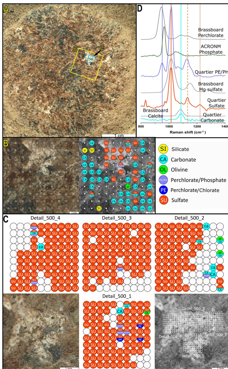
Figure 4. SHERLOC Raman mineral identifications from Quartier. (a) The abrasion patch imaged by WATSON (image ID SIF_0292_0692866773_550FDR_N0090000SRLC00702_0000LMJ01). The yellow box indicates the location of the HDR scan and blue boxes indicate the location of the Detail scans. (b) Colorized (left) and grayscale (right) ACI images (image ID SC3_0293_0692982585_671FDR_N0090000SRLC10600_0000LMJ01) of the region of the abrasion patch bounded by the larger yellow box in panel (a). The white circles in panel B indicate the locations of SHERLOC analysis spots for 0293_Quartier HDR_500_1. Mineral identifications are indicated in the right panel. (c) Colorized (bottom left) and grayscale (bottom right) ACI (image ID SC3_0304_0693962423_667FDR_N0090000SRLC11373_0000LMJ01) images of the region of the abrasion patch where the Detail scans occurred. The white circles on the grayscale ACI image in panel C indicate the locations of SHERLOC analysis spots for four 1 mm 2 Detail scans. The other four subpanels show mineral identifications for Quartier Detail scans. (d) Representative Raman spectra of minerals detected with high confidence from the abrasion patch and spectra of mineral standards collected on the SHERLOC Brassboard instrument at JPL. Vertical lines represent peak centers. Spectra are offset along the y-axis for clarity.
