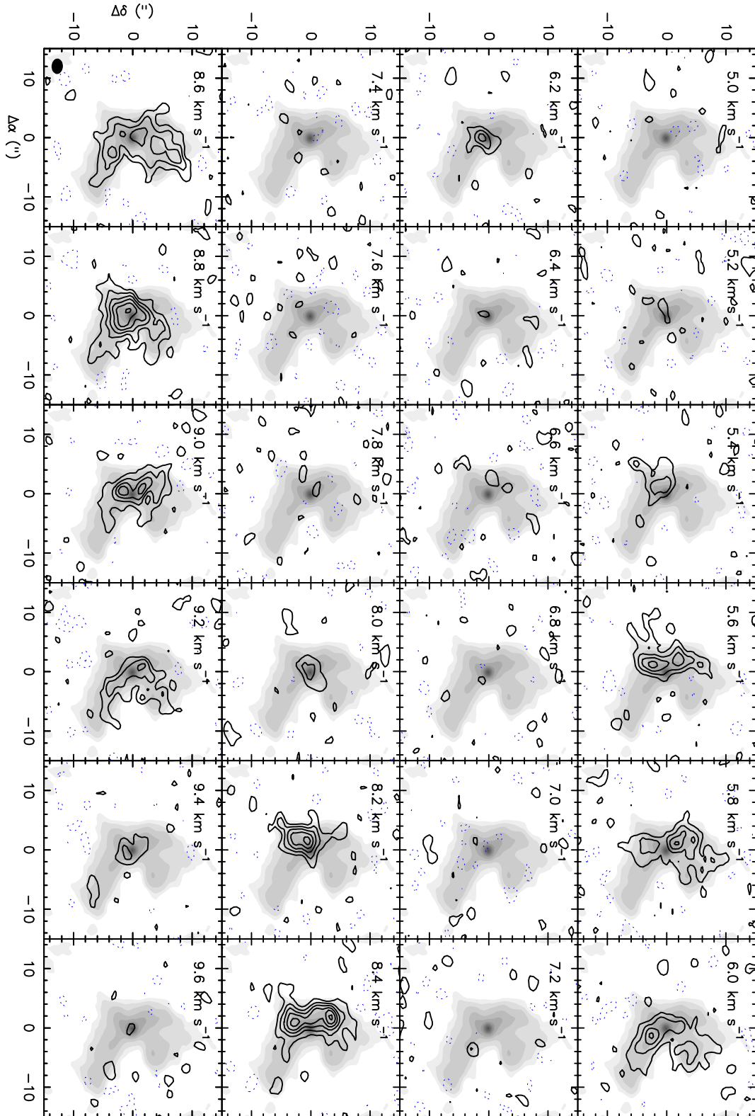
Fig. B.1: Contour channel maps of the C^{17}O (1-0) emission showing the two main hyperfine components, overlapped with the gray scale image of the 1.3 mm dust emission. Contours are -4 , -2 , and from 2 to 18 by steps of 2 times the rms noise of the channel maps, 10 \text{ mJy Beam}^{-1} . The synthesized beam is shown in the bottom left panel as a filled ellipse. The v_{\text{LSR}} channel velocities are shown in the top left part of the panels.
