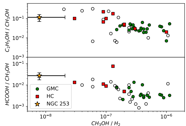
Fig. 12. Abundances of \text{C}_2\text{H}_5\text{OH} and \text{HCOOH} relative to \text{CH}_3\text{OH} towards the NGC 253 CMZ (orange star), compared to those measured towards Galactic hot cores (red squares; Ikeda et al. 2001) and Galactic Center giant molecular clouds (green circles; Requena-Torres et al. 2006). Upper limits to \text{C}_2\text{H}_5\text{OH} and \text{HCOOH} are represented by open symbols.
