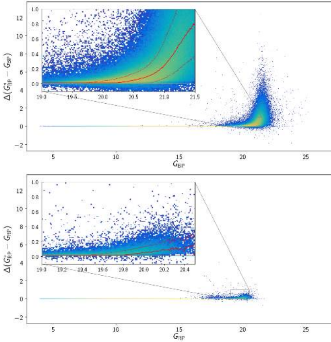
Fig. 27. Change in the G_{\text{BP}} (top panel) and G_{\text{RP}} (bottom panel) magnitude when removing the 1 \text{ e}^{-\text{s}^{-1}} flux threshold vs. G_{\text{BP}} and G_{\text{RP}} magnitude respectively for the sample of \approx 3.4 million nearby sources. The insets show a zoom of the transition region where the discrepancy between the two magnitudes becomes significant. The solid red lines show the median of the residual distribution, and the two red dashed lines show the 84th and 16th percentiles.
