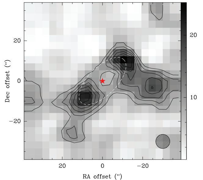
Figure 3. ACA+TP velocity-integrated intensity map of CO J = 2 \rightarrow 1 towards AG Car, in the velocity range (+29, +36) \text{ km s}^{-1} . Contours start at 8 \text{ K km s}^{-1} in steps of 2.5 \text{ K km s}^{-1} . The red marker indicates the position of the star, and the hatched circle in the bottom right corner represents the ACA synthesized beam size. The dashed ellipse represents the ellipse used for the fitting.
