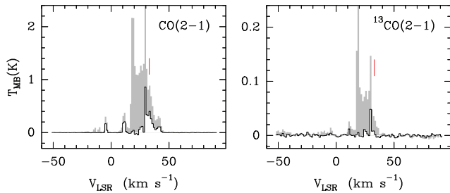
Figure 2. Interferometric filtering towards AG Car. Left-hand panel: CO J = 2 \rightarrow 1 . Right-hand panel: ^{13}\text{CO} J = 2 \rightarrow 1 . In each panel, feathered ACA+TP (filled) and ACA only spectra (black), averaged within a radius of 20 arcsec from the star, are displayed in the same temperature scale. The red lines indicate the central velocity of the component likely associated with the star.
