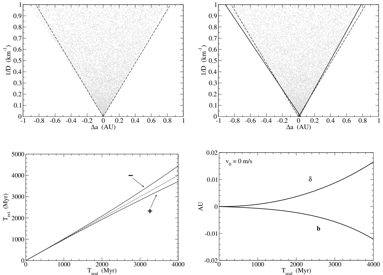
Figure 4. Top: deformation of the V-shape borders due to the acceleration/deceleration of the Yarkovsky drift rate in our reference simulation. T_{real} = 4 Gyr in order to make the effect more visible. The two dashed lines represent the expected borders of the V-shape if the semimajor axis drift rate had been strictly constant, while the solid lines represents the best fit lines of the V-shape borders. Bottom left: behaviour of the estimated ages T_{est\pm} versus T_{real} computed according to the definition explained in the text, for the reference simulation. Bottom right: V-base size b and relative centre of the V-base \delta versus real age T_{real} , for the reference simulation.
