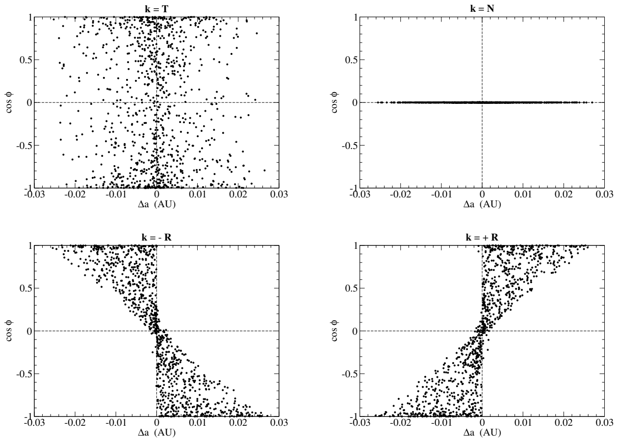
Figure 9. Spin-velocity field with \theta_h = 0 and \eta_s = 0 . The plots show the \cos \phi versus \Delta a for different directions of the symmetry axis \hat{k} : \hat{k} = \pm\mathbf{T} (top left), \hat{k} = \pm\mathbf{N} (top right), \hat{k} = -\mathbf{R} (bottom left) and \hat{k} = +\mathbf{R} (bottom right).
