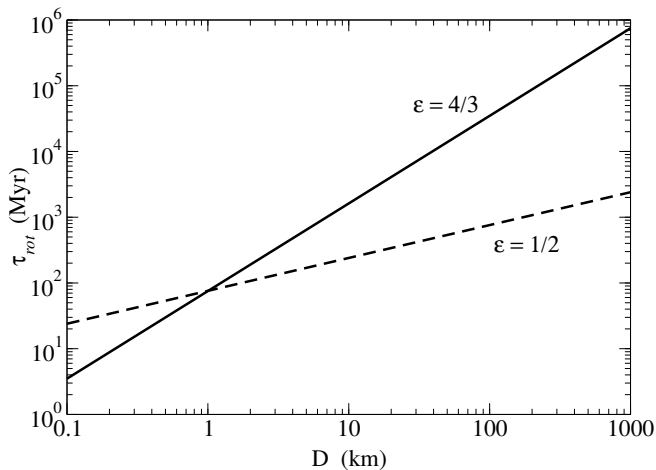
Figure 3. Characteristic time of rotational axis collisional re-orientation versus diameter for Main Belt Asteroids, according to the model by Farinella et al. (1998).
