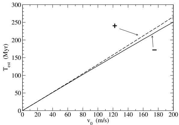
Figure 6. Estimated ages (solid line: T_{est-} ; dashed line: T_{est+} ) versus v_0 , for a not yet evolved asteroid family ( T_{real} = 0 ), characterized by a non null velocity field.
