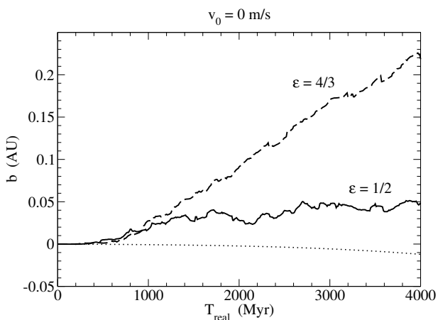
Figure 17. Value of the V-base versus T_{real} for an asteroid family affected by spin reset (solid line \epsilon = 1/2 , dashed \epsilon = 4/3 , dotted line no spin reset).
