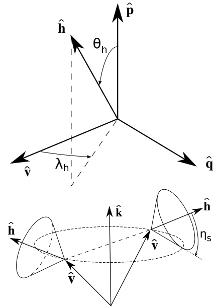
Figure 1. Auxiliary unit vectors used to describe the direction of the spin. At the top the orthonormal axes, defined for a particular fragment, with respect to the direction \hat{\mathbf{h}} of the mean spin axis is defined: the unit vector \hat{\mathbf{v}} along the ejection velocity, the unit vector \hat{\mathbf{p}} normal to the plane containing \hat{\mathbf{v}} and the global symmetry axis of the spin-velocity field \hat{\mathbf{k}} , and \hat{\mathbf{q}} = \hat{\mathbf{p}} \times \hat{\mathbf{v}} . The spin direction for a particular fragment is randomly generated inside a cone of semi-aperture \eta_s around \hat{\mathbf{h}} (bottom).
