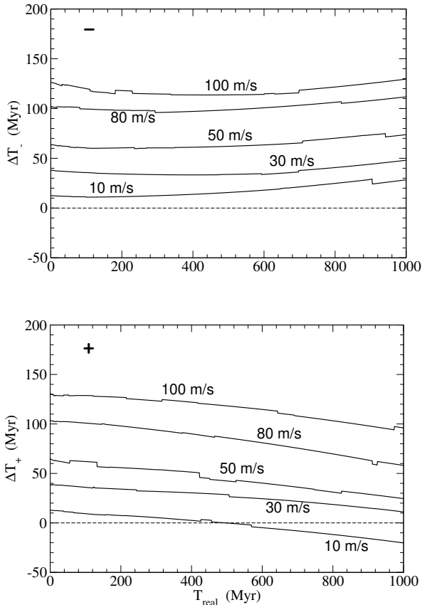
Figure 8. Top: bias of estimated age versus real age for isotropic families with different values of v_0 , obtained from the inverse slope of the V-shape inner border. Bottom: the same but obtained from the outer border.
