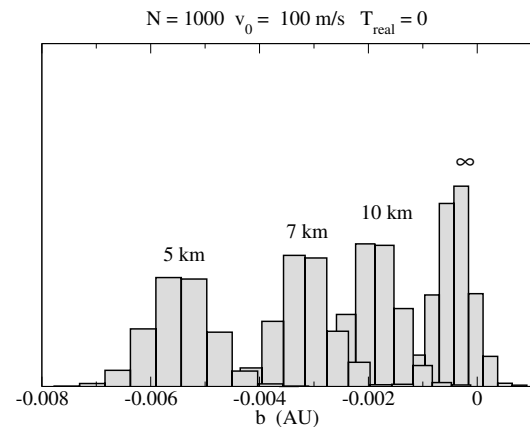
Figure 13. Distributions of the V-base b at T_{real} = 0 , for 1,000 asteroid families with v_0 = 100 m/s consisting of 1,000 members each. The numbers on top of each histogram are the corresponding values of the limit diameter D_{lim} .
