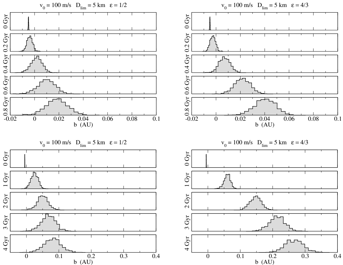
Figure 18. Evolution with time of the distribution of the V-base size b for a set a 1,000 asteroid families affected by an initial reaccumulation and spin reset in the post-formation phase. The break-up parameters are v_0 = 100 m/s and D_{lim} = 5 km. The exponent of the spin reset is \epsilon = 1/2 at left and 4/3 at right. Top: evolution during the first 800 Myr. Bottom: evolution up to 4 Gyr.
