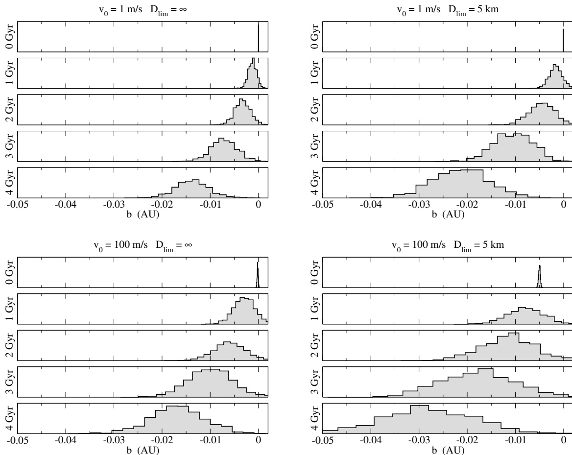
Figure 14. Evolution with time of the statistical distribution of the size of the V-base. Two different sizes of the ejection velocity field are taken into account ( v_0 = 1 m/s at the top, and v_0 = 100 m/s at the bottom). Left: evolution without initial gravitational reaccumulation. Right: case with reaccumulation with limit diameter D_{lim} = 5 km. The number of family members is 10,000.
