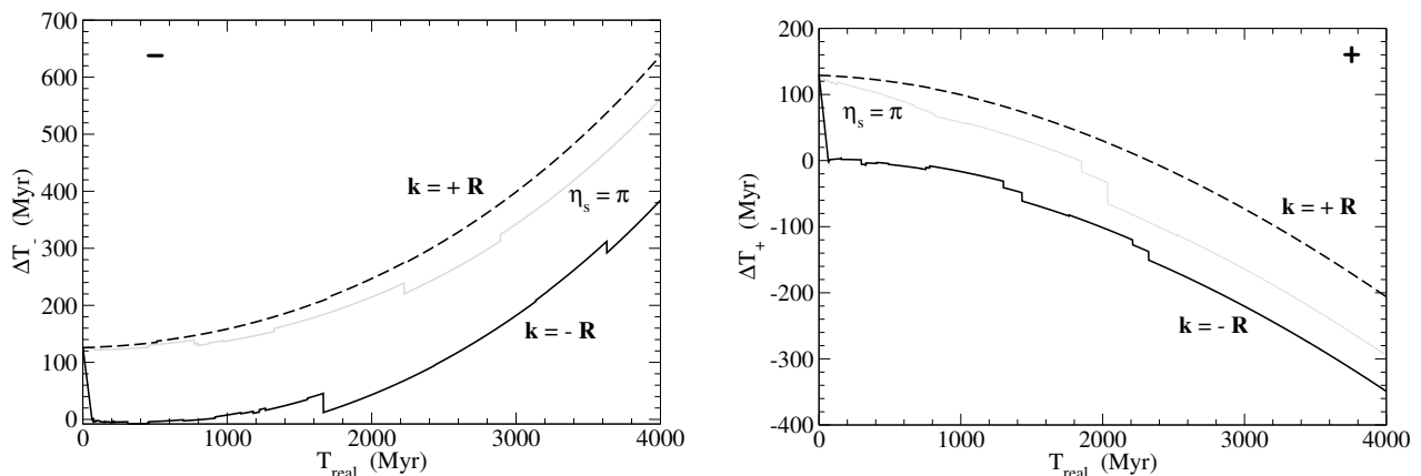
Figure 10. Evolution of the bias \Delta T_{\pm} for a fully isotropic family (null correlation, grey line), a spin-polarized family with \hat{k} = +\hat{\mathbf{R}} (positive correlation, dashed line), and a spin-polarized family with \hat{k} = -\hat{\mathbf{R}} (negative correlation, solid line).
