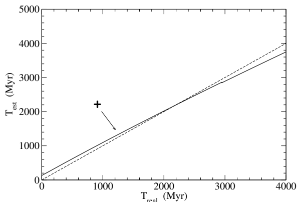
Figure 7. Evolution of an isotropic family with v_0 = 100 m/s. Top: T_{est-} versus T_{real} . Bottom: T_{est+} versus T_{real} . The dashed line represents function T_{est\pm} = T_{real} .
