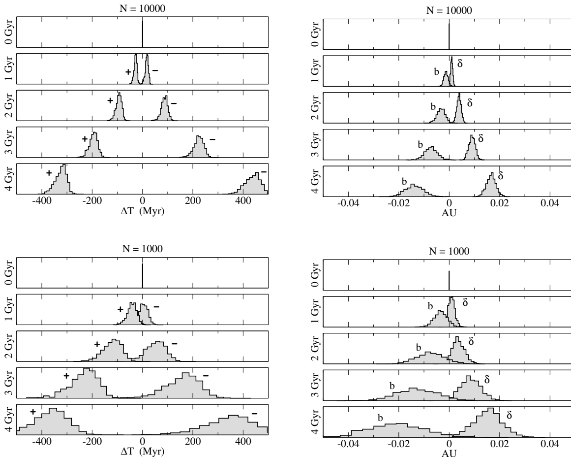
Figure 5. Reference simulation: statistical distributions of the age estimation bias \Delta T_{\pm} = T_{est\pm} - T_{real} (left), and statistical distributions of the V-base size b and of the relative centre \delta of the V-base (right). The two cases of 10,000 members (top) and 1,000 members (bottom) are displayed.
