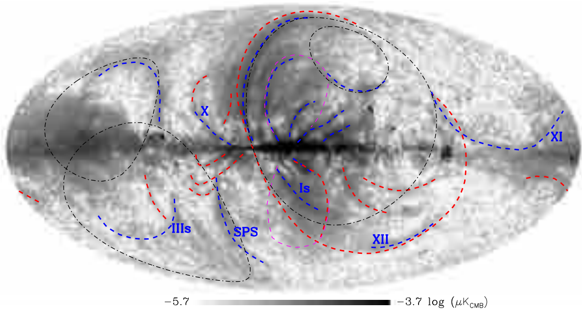
Fig. 22. Synchrotron polarization amplitude map, P = \sqrt{Q^2 + U^2} , at 30 GHz, smoothed to an angular resolution of 60' , produced by a weighted sum of Planck and WMAP data as described in Planck Collaboration XXV (2016) . The traditional locii of radio loops I–IV are marked in black, a selection of the spurs identified by Vidal et al. (2015) in blue, the outline of the Fermi bubbles in magenta, and features discussed for the first time in Planck Collaboration XXV (2016) in red. Our measured outline for Loop I departs substantially from the traditional small circle.
