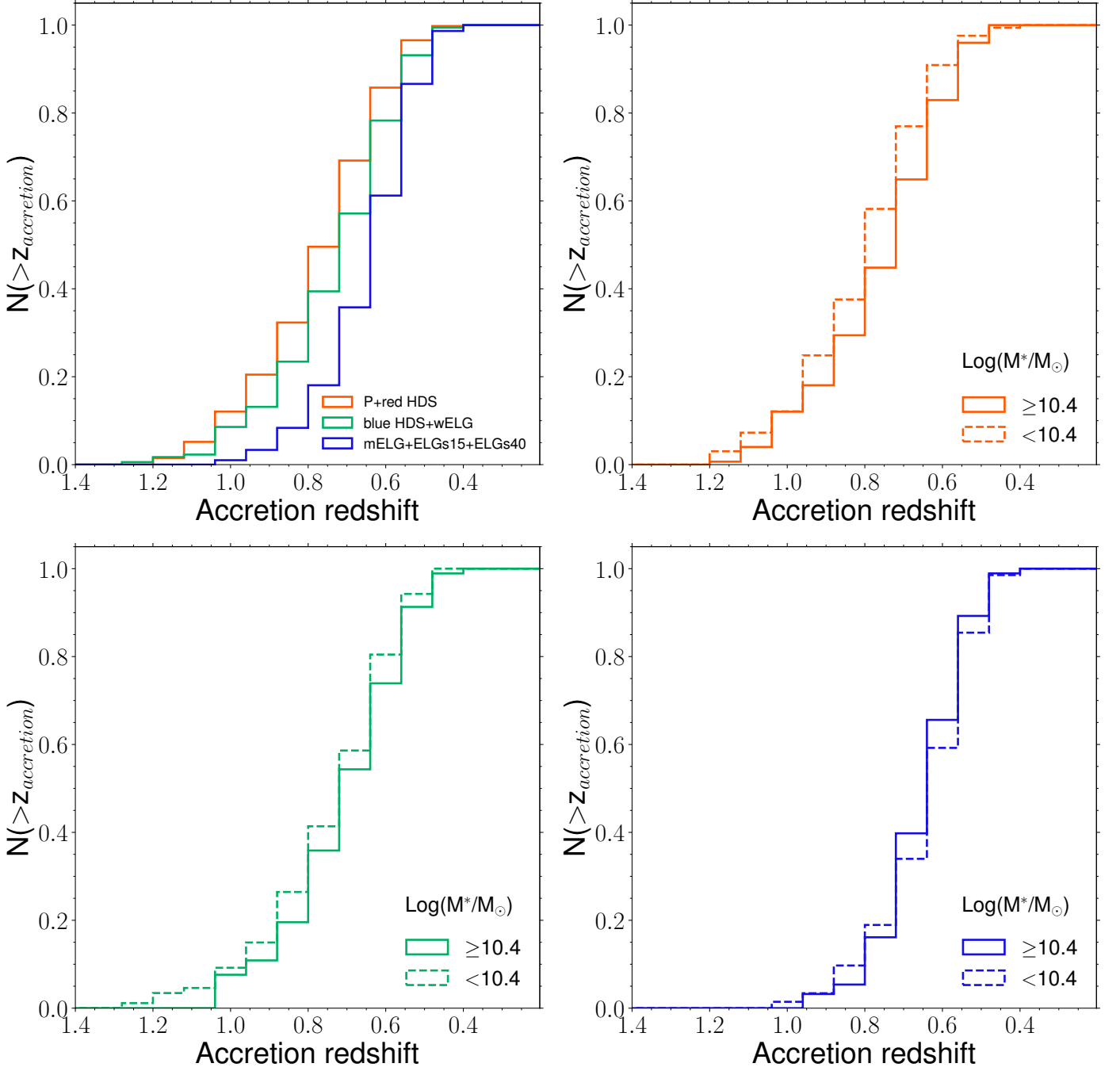
Fig. 20: Upper left panel : cumulative distribution of the accretion redshift, z_{\text{accr}} , for galaxies with different spectral types: passive + red post-starbursts (orange), blue post-starbursts + weak emission lines (green) and strong emission lines (blue). The other three panels show the same distribution separated into high and low mass bins (using as a threshold \text{Log}(M^*/M_{\odot})=10.4 ), for the corresponding (colour coded) galaxy spectra types.
