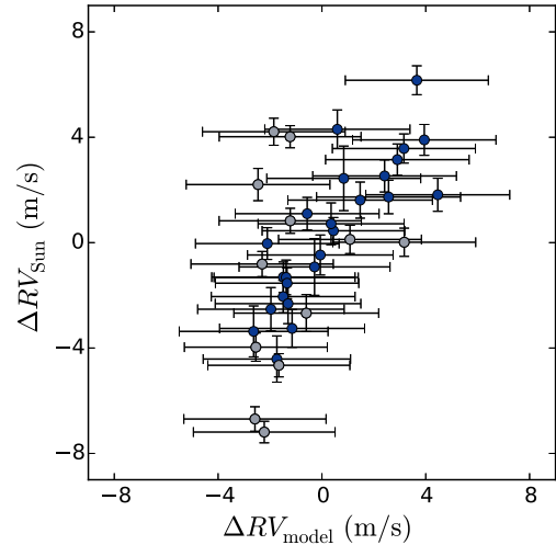
Figure 9. HARPIS RV variations of the Sun as a star versus our model derived from SDO/HMI images. Observations from the first part of the run are highlighted in a lighter shade.
