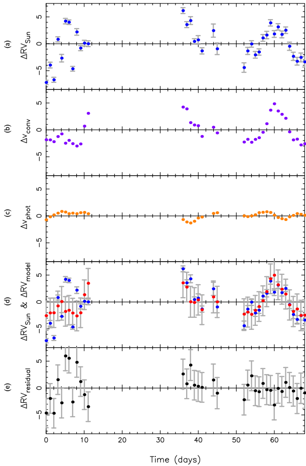
Figure 8. (a) HARPIS RV variations of the Sun as a star, \Delta RV_{\text{Sun}} . (b) Scaled basis function for the suppression of convective blueshift, \Delta \hat{v}_{\text{conv}} , derived from SDO/HMI images. (c) Scaled basis function for the rotational Doppler imbalance due to spots and faculae, \Delta \hat{v}_{\text{phot}} . (d) Total RV model, \Delta RV_{\text{model}} (red/lighter shade, with errors including additional variance s ), overlaid on top of the HARPIS RV variations (blue/darker shade points). (e) Residuals obtained after subtracting the model from the observations. All RVs are in \text{m s}^{-1} . Note that the scale of the y-axis is different from that used in Fig. 2. The values of these nightly binned time series are provided in the Supplementary Files available online.
