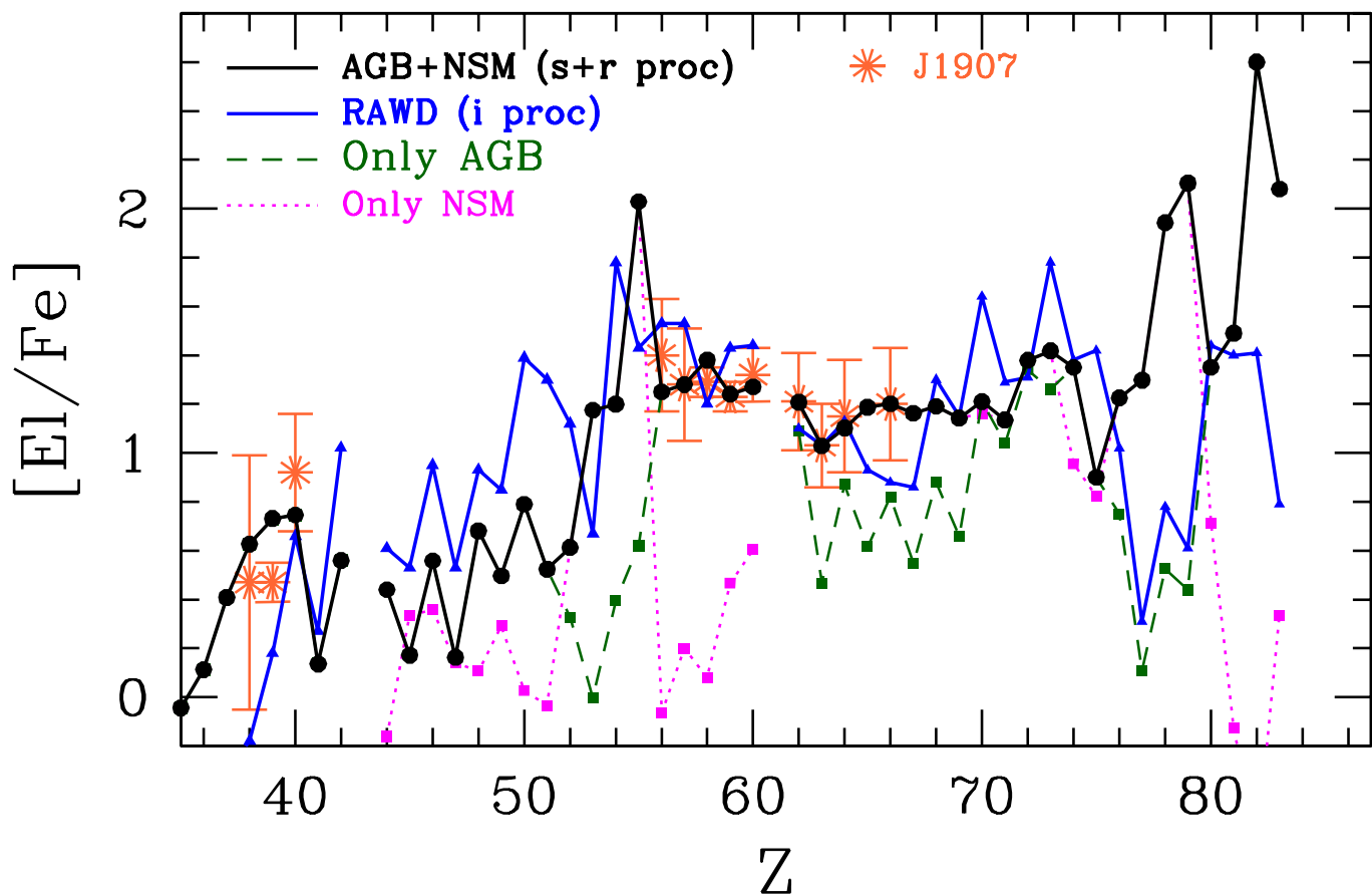
Fig. 7. The abundance pattern of J1907 compared with yields from a NMS (magenta dotted curve), an AGB star (green dashed curve), a combination of them (black solid curve) and RAWDs (blue solid curve). See text for details.
