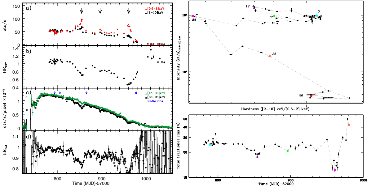
Fig. 1. Left: XRT light curves in the 0.5–2 keV and 2–10 keV energy ranges, extracted by pointing (panel a ), plotted with the corresponding hardness ratio (panel b ). In panel c , we show the 15–30 keV and 30–90 keV light curves observed by BAT, with a 1-day binning time, and the related hardness ratio (panel d ). In the XRT light curve, three strong peaks (black arrows) in correspondence to dips in the BAT light curve and in the hardness ratios have been observed. These indicate softening in the X-ray spectra. Upper Right: Hardness-Intensity Diagram. The outburst has been observed by XRT when GRS 1716–249 was at the top-right side of the pattern (cyan dot), then it evolves along the horizontal branch (purple triangle). It reaches the softest state (magenta square) and then takes a diagonal trajectory (orange dot) on its return to the hard state (red dot), before going in quiescence. The magenta square, purple triangle, and green diamond correspond to the softest points in each of the three softening episodes. Lower Right: XRT fractional rms evolution. The soft points observed in the HID correspond to fractional rms values typical of the HIMS (10%–30%, Muñoz-Darias et al. 2011).
