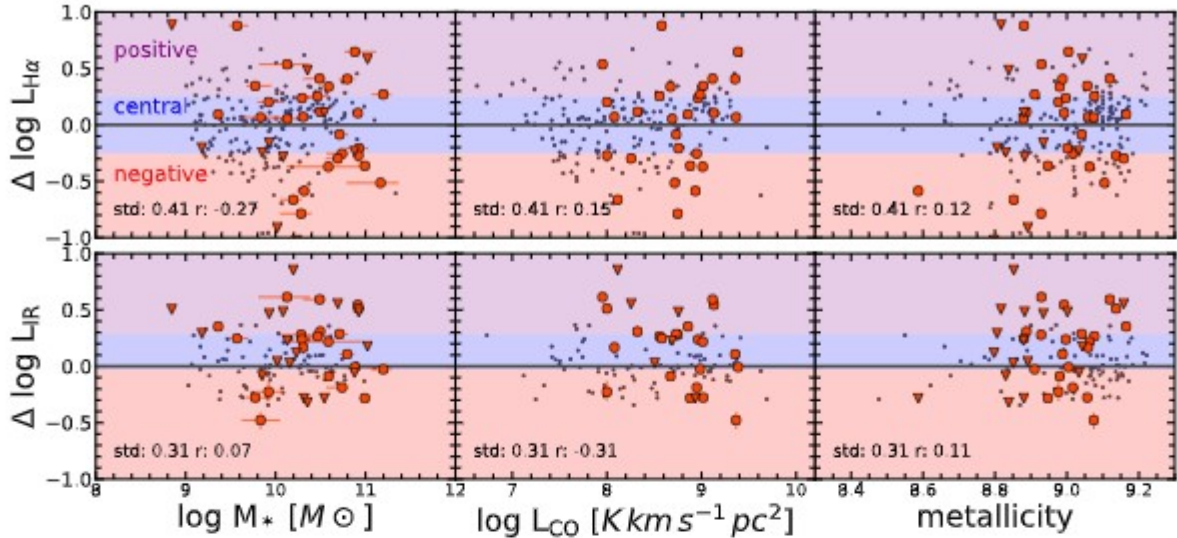
Fig. 7. Difference between measured and expected H \alpha (upper panels) and FIR luminosity (lower panels) as a function of stellar mass, CO(1–0) luminosity and 12 + \log(O/H) ionized gas metallicity. Here we used our more complex model (Eqs. (1) and (2)) to predict the SFR-sensitive luminosities. The black dots are the data from our xCG training sample and the red symbols are the CARS data with triangles indicating upper limits. The colored bands (red, blue and purple) define three bins in residual luminosity as discussed in the text and used for Fig. 8.
