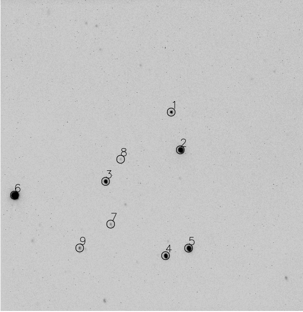
Fig. A.1. Field of ISO-Chal 52 as observed by ROSS2 camera with the i' filter. The identification code (ID in Table A.1) is written next to the stars for which we extracted magnitudes. ID = 1 for ISO-Chal 52.
