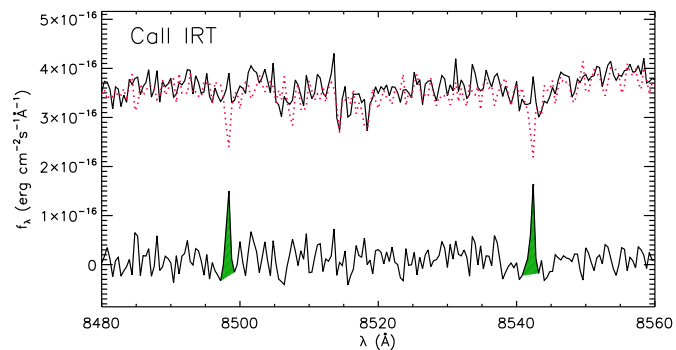
Fig. C.2. X-shooter spectrum of ISO-ChaI 52 in the region of Ca II IRT (solid black line) along with the inactive template (dotted red line). The difference between observed and template spectrum is shown in the bottom of the box, along with the residual emission in the line cores (hatched green areas).
