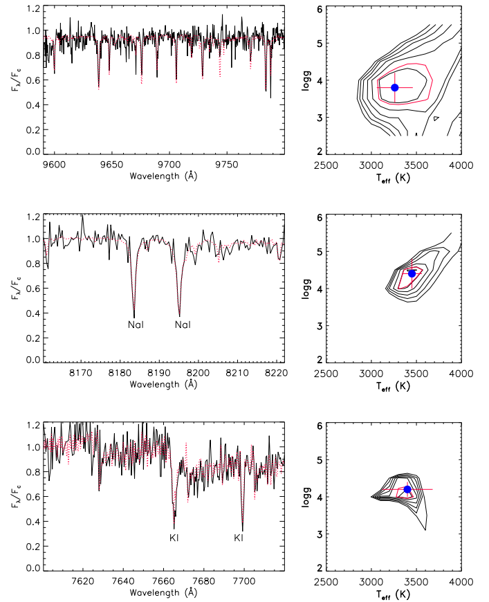
Fig. B.1. Left panels: continuum-normalized VIS X-shooter spectrum of ISO-Chal 52 in three regions (full black lines) with the best-fitting synthetic spectrum overplotted (dotted red lines). Right panels: \chi^2 contour maps in the T_{\text{eff}} – \log g plane. In each panel, the 1\sigma confidence level is denoted by the red contour. The best values and error bars on T_{\text{eff}} and \log g are also indicated.
