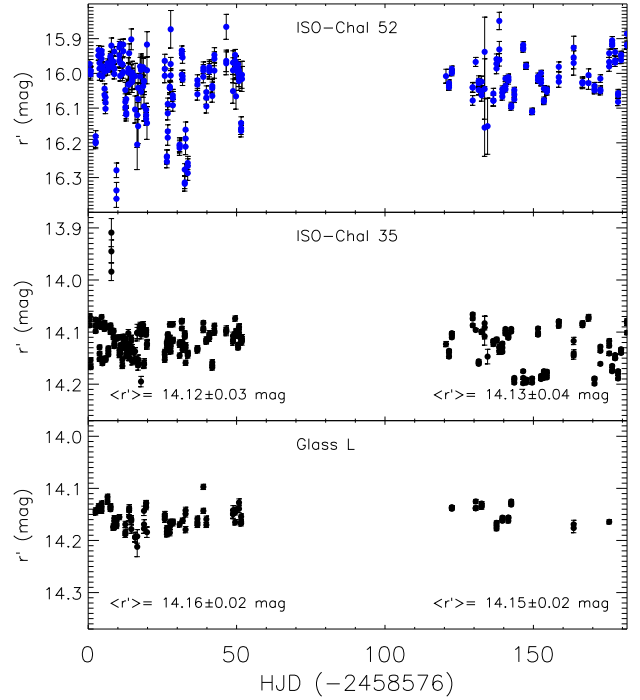
Fig. A.2. ROSS2 r' light curve of ISO-Chal 52 (top panel), ISO-Chal 35 (middle panel), and Glass L (bottom panel). We have used 2MASS J11042217–7741319 (star 2) for the first two stars and Glass M (star 5) for the latter as comparison stars, adopting the magnitudes listed in Table A.1. The average magnitudes of the last two stars and their rms scatter are provided in the respective panels for the two data segments.
