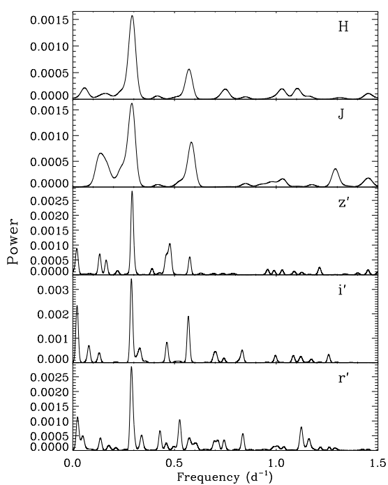
Fig. C.3. Cleaned periodograms for the photometric data of ISO-ChaI 52 in the HJz'i'r' bands (from top to bottom). The highest peak in each band corresponds to a period of about 3.45 days.
