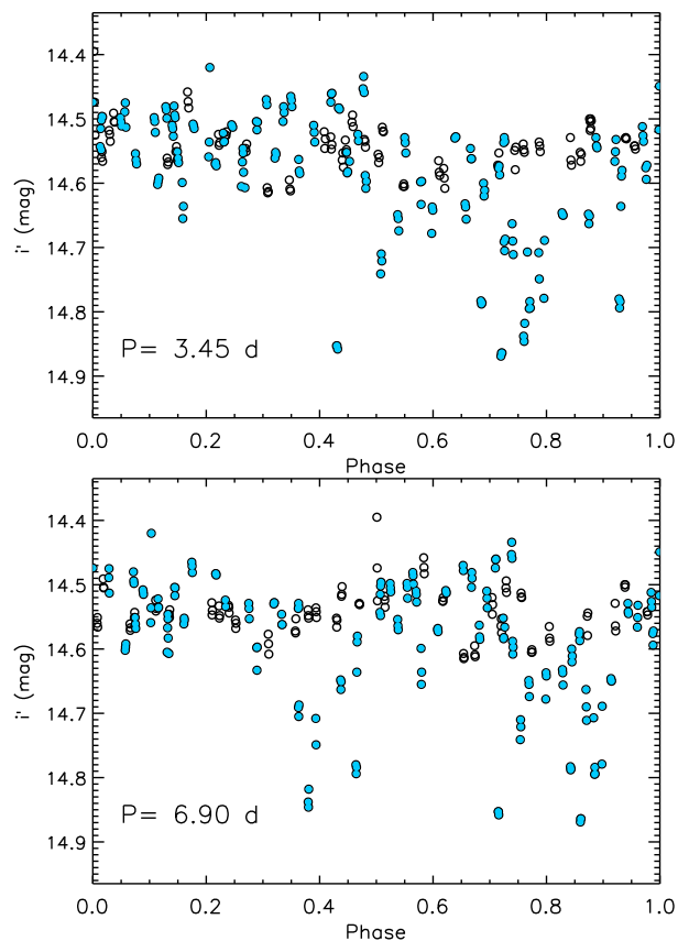
Fig. C.4. Light curve in the i' band folded in phase with the period of 3.45 days (upper panel) and 6.9 days (lower panel). Filled dots refer to the data acquired before the end of May 2019 (JD < 2458630), and open dots are related to the second part of the data (August–October 2019).
