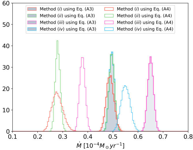
Fig. A.1. Mass-loss rate distribution for Cygnus OB2 considering the sample of stars investigated by Wright et al. (2015) . The stellar parameters are estimated using four different recipes, from (i) to (iv), and for each one the mass-loss rate is estimated using both Equation (A.3) and (A.4). All estimates neglect the contribution due to WR stars.
