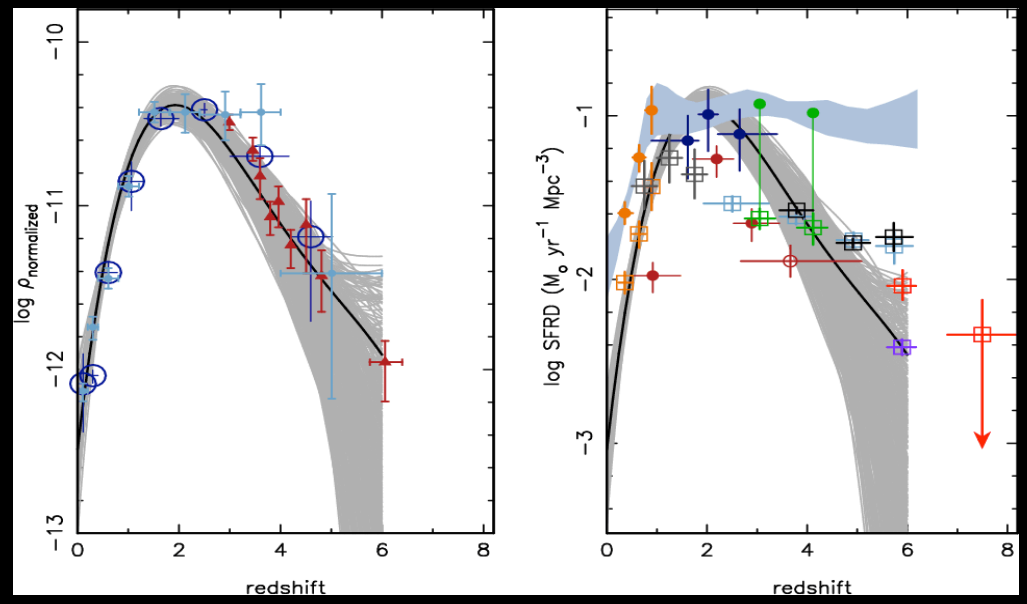
QSO space density
