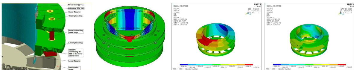
Figure 12: (A) Overview of the mechanical set-up of the Mirror Shell (MS), the shell Support System (SSS) and the Invar Spoke Wheel (ISW). (B) The OOR of the MS related to the lowest MS frequencies. The isocontours of the radial displacement component of the whole assembly under lateral gravity (C) and under axial gravity (D)
