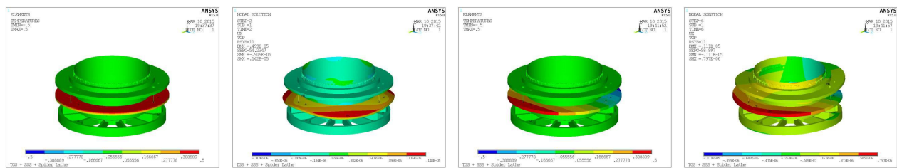
Figure 13: Examples of temperature gradients effects on the ISW + SSS + MS system. (A) A temperature gradient (1°C along the total ring thickness), in axial direction, is considered on the lower glass rings. (B) Radial displacement isocontours of the MS. (C) A temperature gradient of 1°C, in lateral direction, is considered on the lower glass rings. (D) Deformed shape with radial displacement isocontours quoted in meters.
