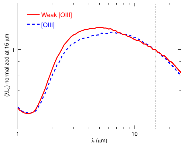
Fig. 4. Average SEDs corresponding to WISE photometry of the WISSH [OIII] (dashed blue line) and Weak [OIII] samples (red line), normalized at 15 \mu\text{m} (dot-dashed line).
