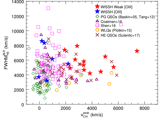
Fig. 9. \text{FWHM}_{\text{Hg}}^{\text{BLR}} as a function of v_{\text{CIV}}^{\text{peak}} for the WISSH sample, compared to PG QSOs from Baskin & Laor (2005) and Tang et al. (2012) (green diamonds), WLQs from Plotkin et al. (2015) (orange circles), SDSS QSOs from Shen (2016) and Coatman et al. (2016) (magenta squares and purple triangles, respectively) and HE QSOs from Sulentic et al. (2017).
