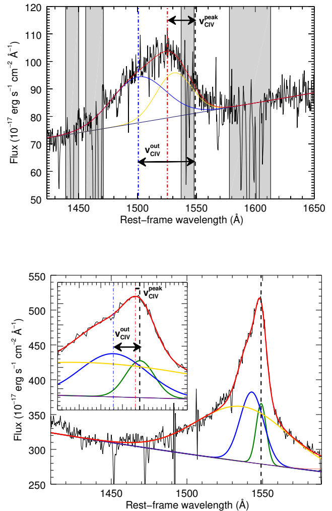
Fig. 2. Parametrization of the CIV emission line profile of the Weak [OIII] quasar J1422+4417 (Upper panel) and the [\text{OIII}] quasar J0745+4734 (lower panel). In both panels the red, yellow and blue curves refer to the best-fit of the spectrum, virialized component and outflow component of the CIV emission line, respectively. The black dotted line indicates the \lambda_{\text{CIV}} at 1549 \text{\AA} . The red dotted-dashed line denotes the peak of the CIV emission line and v_{\text{CIV}}^{\text{peak}} represent its velocity shift with respect to the systemic \lambda 1549 \text{ \AA} . The blue dotted-dashed line indicates the peak of the outflow component and v_{\text{CIV}}^{\text{out}} is its velocity shift with respect to the systemic redshift. In the lower panel the green curve refers to an additional Gaussian component required by the fit, in order to better described the CIV profile in this QSO.
