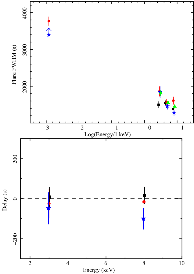
Figure 11. ( Top panel ) Flare duration ( FWHM ) at various energies of the three brightest XMM-Newton flares, VB1, VB2, VB3 and of the combined XMM-Newton flare light curve are shown with back squares, red circles, blue stars and green triangles, respectively. The flare duration is computed in the 2-4, 4-6 and 6-10 keV energy bands (the points are slightly shifted for display purposes). Flares are typically shorter at higher energies. We also show the duration of VB2 (as observed in the L' band, see §5.2) and the lower limit on the duration of VB3 (as observed with SINFONI ). The flare durations in the NIR band connect with the extension of the trend observed in X-rays. ( Bottom panel ) Peak occurrence delay, between different energies (same energy bands as above) for the three very bright flares observed by XMM-Newton . The delays are computed as the best fit peak value of the Gaussian at each energy minus the same value observed in the 4-6 keV band. Colour code as before.
