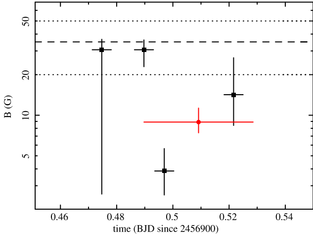
Figure 9. Evolution of the strength of the magnetic field (in Gauss) during and after the flare VB3, in the PLCoolEv model. The black squares show the magnetic field strength during IR1 to IR4. The red circle shows the measurement of the average magnetic field during the entire duration of the X-ray flare VB3 (under the assumption of a constant escape time of t_{esc} = 300 s). The dotted lines indicate the typical range of magnetic field strengths during quiescence ( B \sim 20 - 50 G). The dashed line shows the magnetic field strength ( B \sim 36 G) corresponding to a cooling break within the narrow SINFONI band. The flat NIR slopes observed at all times during the flare suggest B < 36 G, while the steep NIR slope observed after the VB3 flare (during IR5, IR6 and IR7) suggest B > 36 G. The error bars correspond to the 1-sigma uncertainties as derived from the confidence contours shown in Fig. 8. No evidence for a cut off at or below the X-ray band is observed during IR4, therefore the associated measurement is valid under the assumption that the cut off is at energies higher than the X-ray band. Would this assumption be invalid, such constraint should be considered as an upper limit.
