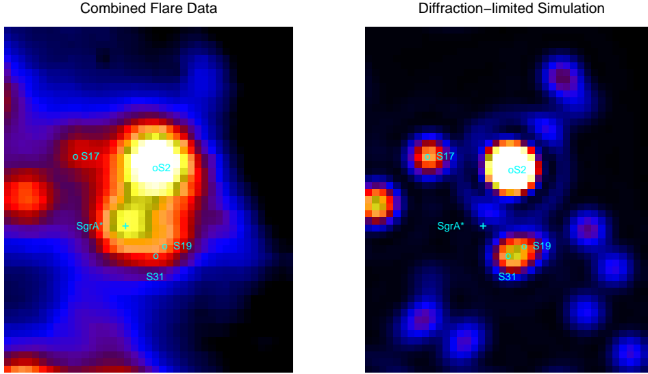
Figure 2. The GC as seen with SINFONI (each image is 0.51'' \times 0.61'' ). The image on the left is the collapsed image from the spectral range 2.25\text{--}2.35 \mu\text{m} for the seven data cubes combined. The image on the right is a diffraction-limited simulated image of the locations of the S-stars in the GC. In both images the location of Sgr A* is indicated with a cross, and the four stars included in our Gaussian fits for spectrum extraction are labeled with circles. The flare is clearly visible above the background in the left image.
