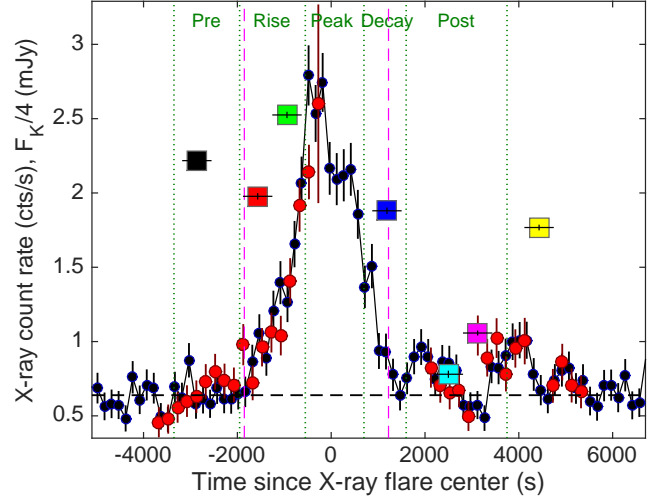
Figure 5. The black and red points show the XMM-Newton 2–10 keV (sum of the three EPIC cameras) and NuSTAR 3–20 keV light curve of Sgr A*’s flare VB3 (Ponti et al. 2015), respectively. A constant rate of 0.13 \text{ cts s}^{-1} has been subtracted from the NuSTAR light curve for display purposes, to take into account the different contribution of the diffuse and quiescent emission (gaps in the NuSTAR light curve are due to Earth occultation). The squares show the extinction corrected SINFONI light curve of Sgr A* during the VB3 flare. Each point corresponds to a NIR spectrum integration time of 600 s. The y-axis reports the observed renormalised (divided by 4 for display purposes) flux density at 2.2 \mu\text{m} in mJy units. The black dashed line indicates the level of the “non-flare” (quiescent in X-rays) emission. The pink dashed lines indicate the start and end of the XMM-Newton VB3 flare, as indicated by the Bayesian block decomposition (see Ponti et al. 2015a). Excess X-ray emission is observed \sim 2000 and \sim 4000 s after the X-ray flare peak. The dotted green lines show the intervals for the integration of the pre-, rise, peak, decrease and post-flare spectra during VB3. The zero point of the abscissa corresponds to 525831144.7 \text{ s} ( \text{TT}_{\text{TBD}} ) and 2456900.50784 \text{ day} ( \text{BJD}_{\text{TBD}} ), respectively.
