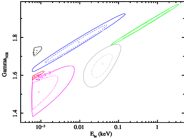
Figure 8. The black, red, green, blue and grey lines show confidence contours of the uncertainty on E_{br} and \Gamma_{IR} for IR1, IR2, IR3, IR4 and the mean spectrum once fitted with the PLCool model, respectively. The dotted and solid lines show the 68 and 90 % confidence contours, respectively. During IR1 and IR2 the cooling break pegs at its lowest value, being located just above the NIR band. Once fitted with the PLCoolEv model, the confidence contours remain unchanged for IR3, IR4 and the mean spectrum, because during these intervals the high energy cut off is at very high energy. The magenta lines show the confidence contours during IR2, when the cut off is observed in the X-ray band. During IR1, the cut off falls between the NIR and X-ray band, therefore the location of the cooling break is unconstrained.
