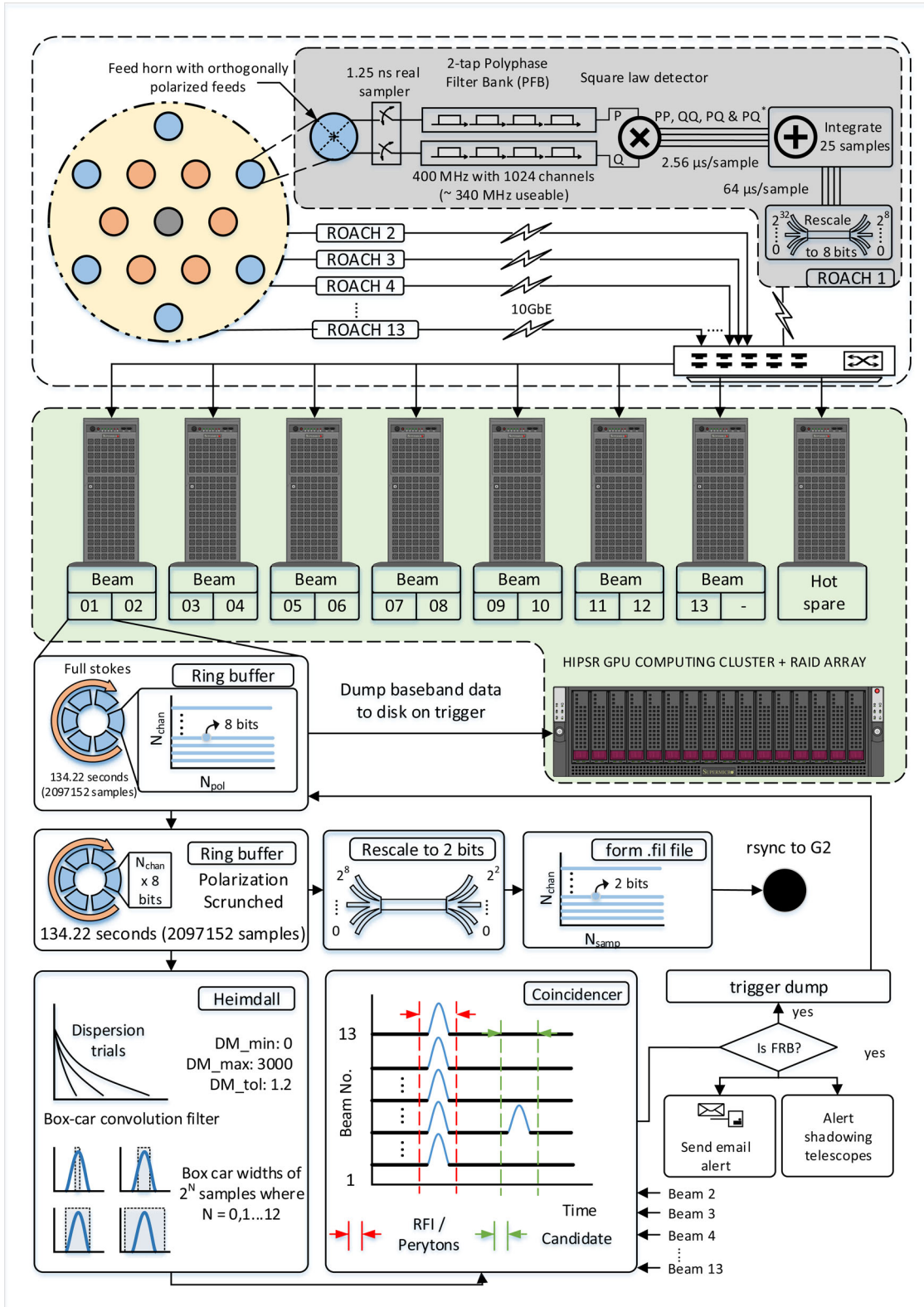
Figure 3. A schematic of the SUPERB acquisition and data analysis pipeline. The topmost block shows the Parkes primary beam (yellow) with the 13-beam pattern of the multibeam receiver overlaid. Each beam is processed separately in the same way (grey block) on a Roach field programmable gate array – Nyquist sampled in two orthogonal polarizations, formed into a filterbank, square-law detected to polarization products and integrated down in time, rescaled from 32 bits to 8, then transferred to a GPU-enabled computing cluster for further searching (green block). The F pipeline single-pulse search happens on these machines – a ring buffer in memory is searched for dispersed pulses satisfying several criteria (see main text) to identify these as FRB candidates. Bona fide FRB candidate information is sent to other telescopes for data dumps (for shadowing telescopes) and/or follow-up.
