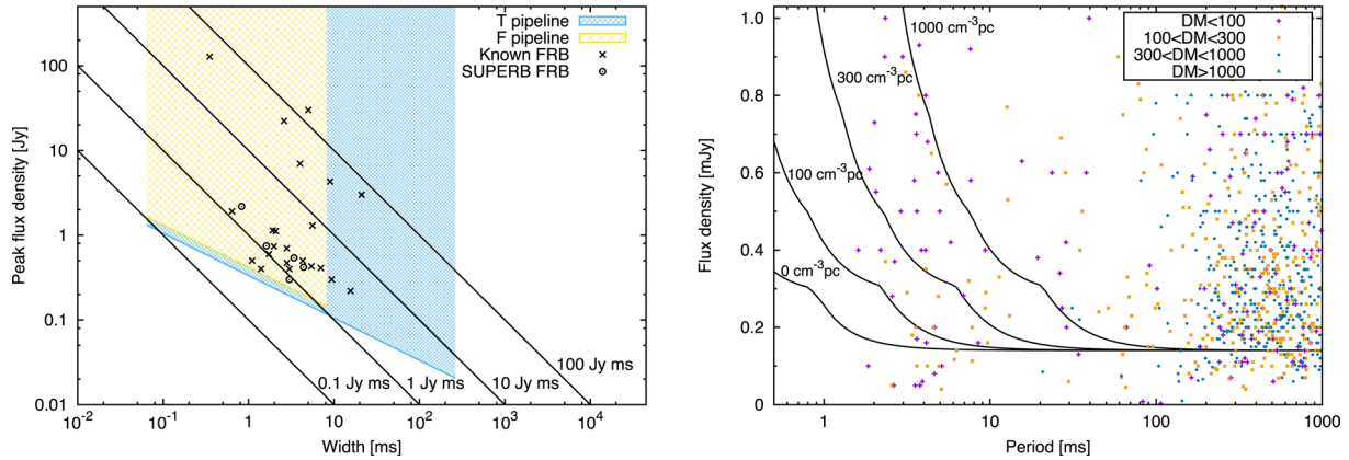
Figure 1. Left: single-pulse search sensitivity plot for the SUPERB survey. Overplotted are the 27 known FRBs with the relevant parameters published, including the five SUPERB discoveries (see the FRB Catalogue of Petroff et al. 2016, Keane et al. 2016 and Paper II for more details). Right: periodicity search sensitivity plot for the SUPERB survey with the known pulsar population overplotted in subgroups (denoted by different symbols and colours) divided by their DM values.
