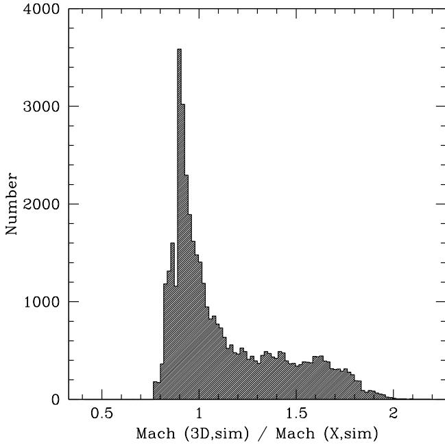
Fig. 7. Distribution of the ratio between the 3D Mach number \mathcal{M}_{3D,sim} and the average X-ray Mach number \mathcal{M}_{X,sim} for five radio relics extracted from our simulations.
