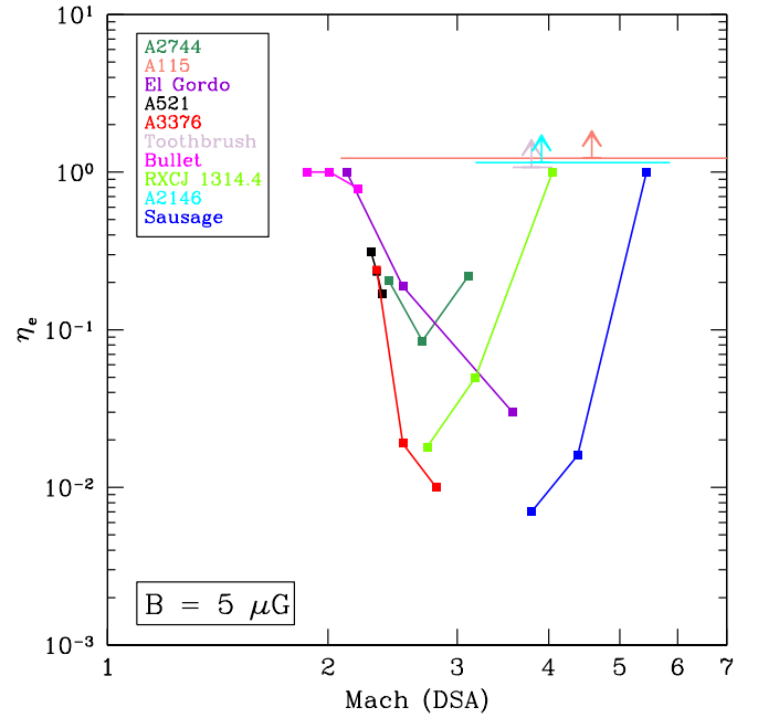
Fig. 8. Electron acceleration efficiency vs. \mathcal{M}_{DSA} obtained for B = 5 \mu\text{G} . For the Sausage relic, f_{DSA} was calculated by assuming \mathcal{M}_X = 2.5 . Upper limits at \eta_e > 1 are slightly offset for display purposes.
