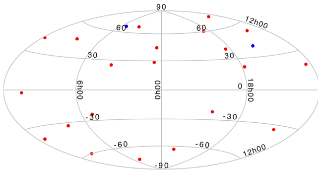
Figure 9. Sky distribution in Galactic coordinates of 23 RRLs for which absolute magnitudes in the V and K bands have been estimated using the BW technique. Red and blue-filled circles show RRAb and RRC stars, respectively.
