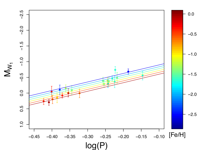
Figure 18. PM_{W_1} distribution of 23 RRLs from our sample, for which absolute M_{W_1} magnitudes were inferred from the model described in Section 4. The lines represent projections of the fit shown in the second portion of Table 4 on to the magnitude–period plane. The colour scale encodes metallicity values measured on the high-resolution spectroscopy metallicity scale.
