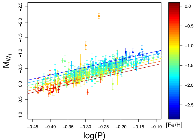
Figure 16. PM_{W_1} distribution of 397 RRLs from our sample, for which absolute M_{W_1} magnitudes were inferred from the model described in Section 4. The lines represent projections of the fit shown in the first portion of Table 4 on to the magnitude–period plane. The colour-scale encodes metallicity values measured on the Zinn & West (1984) metallicity scale.
