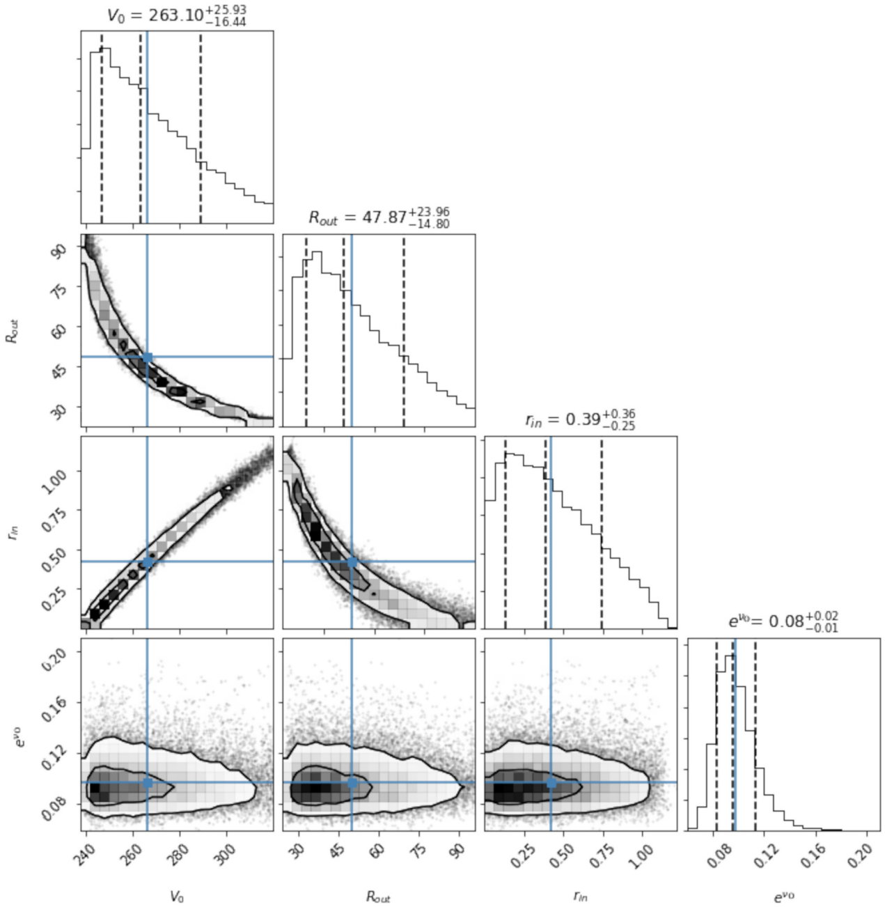
Figure C2. BG parameters corner plot. Same as in Fig. C1.
