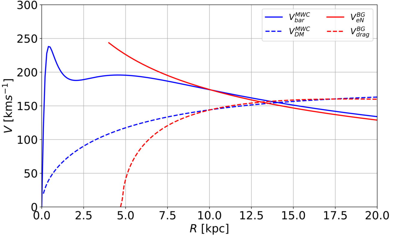
Figure 3. Red and blue colours refer to the BG and MWC model, respectively. Solid lines represent the relativistic effective Newtonian RC, V_{eN}^{BG} , and its analogue for the MWC model, as contributed by the total of baryonic mass. The dashed lines show the MWC halo component alone, and the gravitational dragging contribution to V^{BG} , V_{drag}^{BG} , obtained by subtracting V_{eN}^{BG} from V^{BG} itself (see Section 5 for details).
