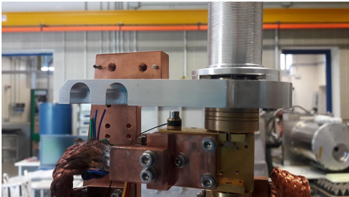
Figure 5. the shimmed configuration as mounted on the CCA (the aluminium support is not fixed yet to the copper vertical support: the gap between the pins (placed in top edge of the copper support) and the aluminium holder was compensated by introducing the two 15 mm straight waveguides.
