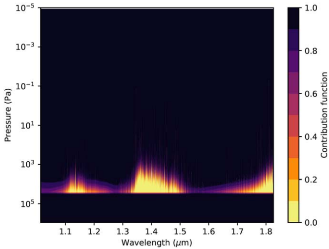
Figure 12. Typical contribution function of our retrievals. We can see the effect of the H 2 O lines. The rise in sensitivity at \approx 10^4 Pa is due to the opaque cloud.
