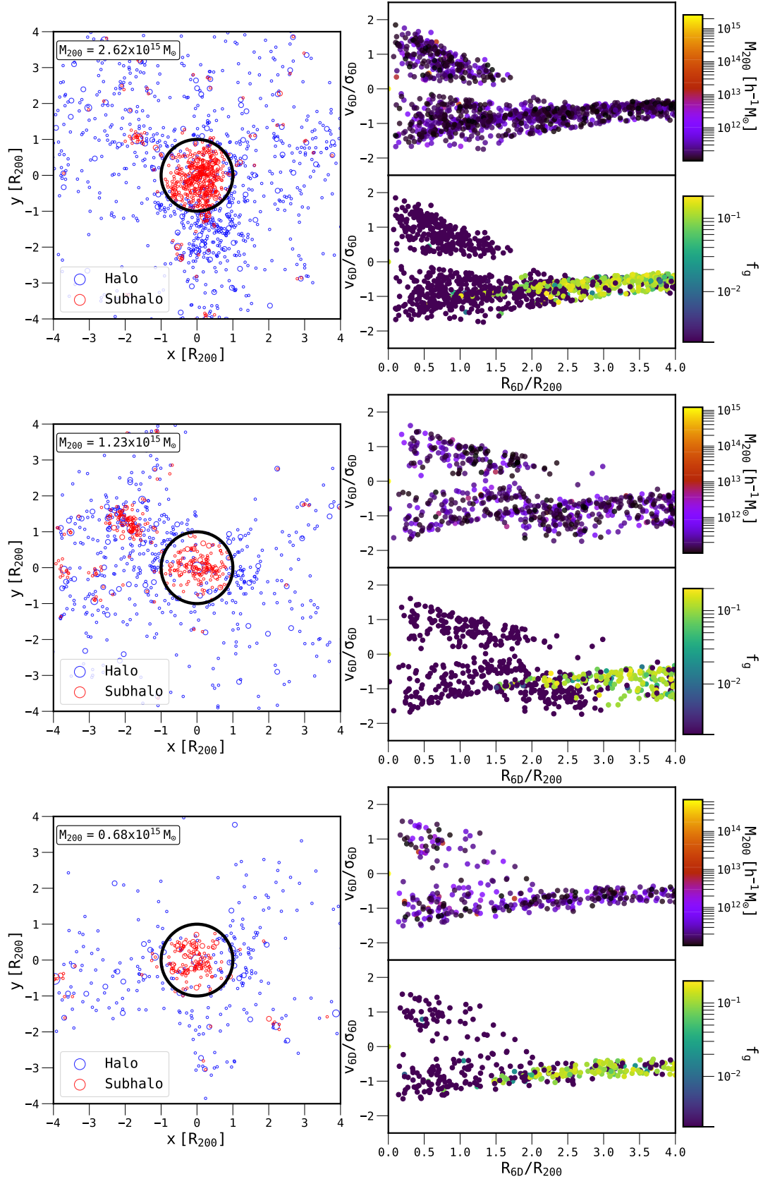
Figure 3. Three sample cluster resimulations from the THETHREEHUNDRED project are shown. For each resimulation, the left panel shows the projected halo and subhalo spatial distributions in blue and red respectively. The black circle indicates where R_{200} of the cluster in the centre is. In the right panels, the 6D phase-space information for all of these haloes and subhaloes can be found. The top and bottom phase-space panel for each region are colour-coded by M_{200} and gas fraction respectively. THETHREEHUNDRED project enables access to this information in a range of cluster environments, and it is apparent in these examples that the halo and subhalo gas fraction may be correlated with phase-space location.
