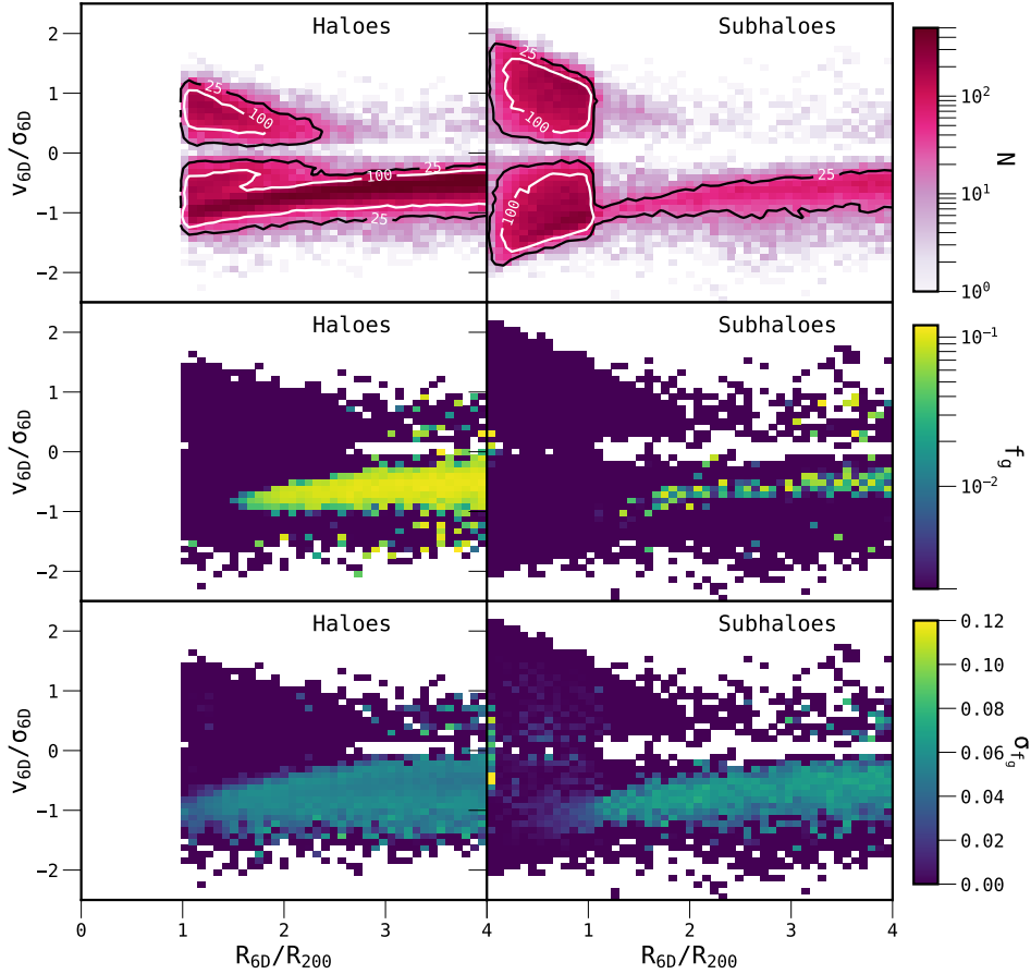
Figure 7. The stacked phase-space planes for all 324 clusters in the THE THREE HUNDRED project, split by subhalo status. The left- and right-hand columns show only haloes and subhaloes respectively in the 6D perspective. The planes are constructed like in Fig. 5. \sim 10 percent of all infalling objects are in the form of subhaloes, which are substantially more gas-poor than haloes in the same phase-space location.
