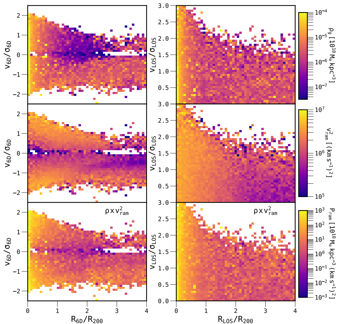
Figure 9. The stacked phase-space planes for all 324 clusters in the THE THREE HUNDRED project, including both haloes and subhaloes. Here, the panels depict the effects of each term in Eq. 4, used for calculating the instantaneous ram pressure. The planes are stacked on a 50 \times 50 grid where the top row is colour-coded by the median local gas density in each bin, the middle row is colour-coded by the median differential velocity between the objects in each bin and their local gas, and the bottom row is colour-coded by the product of the first two rows as calculated by using the method described in Section 2.5. The left and right columns show the 6D and LOS perspectives, respectively. The 6D perspective shows that infalling objects typically experience higher local gas density than the outgoing population, but this is washed out in the LOS perspective. There are distinct regions in the phase-space planes with low v_{\text{ram}}^2 , and these line up well with the regions of high object gas fractions in Fig. 5.
