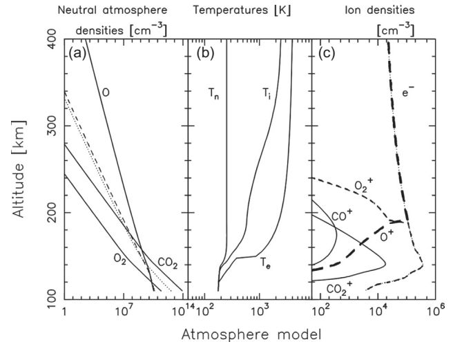
Fig. 18. Dayside upper atmosphere model for Venus. The dotted line (a) represents the \text{N}_2 density and the dashed line the \text{CO} density. In (b) T_n is the neutral temperature, T_i the ion temperature and T_e the electron temperature. In (c) an ion density semi-empirical model is used. This model was computed for F_{10.7} = 80 , latitude: 45^\circ at noon. From Gronoff et al. (2008).
