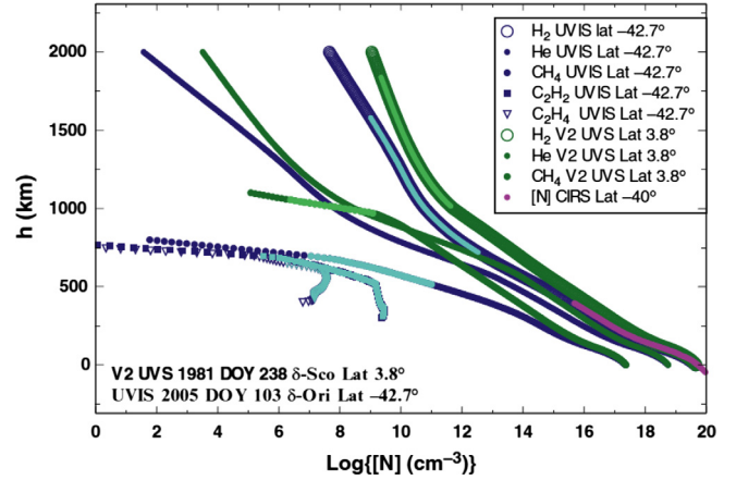
Fig. 4. Density profiles of various components of Saturn's upper atmosphere obtained from forward modelling of the Cassini UVIS \delta -Ori stellar occultation on 2005 DOY 103 at a latitude of -42.7^\circ . From the book Saturn from Cassini-Huygens (M.K. Dougherty et al. eds.), Chapter 8 by Nagy et al. (2009).
