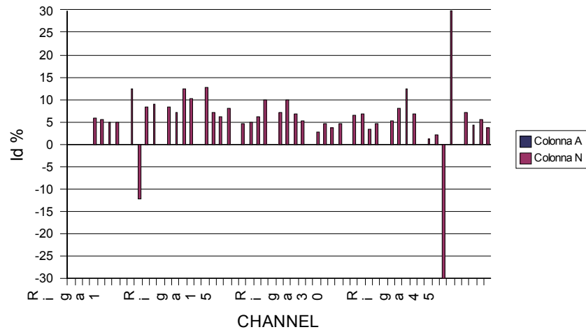
Figure 1 Current consumption of LFI from CRYO-02 respect to average ILT results. Values are expressed in percentage of Id. The hard requirement is +/- 5%. Channel RCA 18 main is here different w.r.t. ILT because it was substituted with the Flight Spare after a failure occurred at phase switch level.
