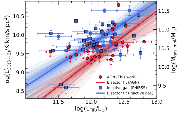
Fig. 2. L'_{\text{CO}} and molecular gas masses as a function of L_{\text{FIR}} for our AGN sample (red circles) and inactive galaxies (blue squares; Tacconi et al. 2018). To display the distribution of the two samples in the plot, we performed a bisector fit by adopting a Bayesian framework (see text). The dispersion of the fits is given by plotting 500 realizations of the bisector fit. Where the fits are better constrained ( \log L_{\text{FIR}}/L_{\odot} = 12.2 ) AGN show CO luminosities 0.43 dex lower than inactive galaxies at the \sim 2\sigma level.
