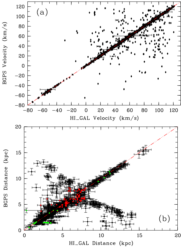
Fig. 11. (a) Velocity (2285 sources) and (b) distance (2050 sources) comparison between paired BGPS and Hi-GAL sources. The red dash-dotted line is the y = x line. Same color coding as in Fig. 10.
