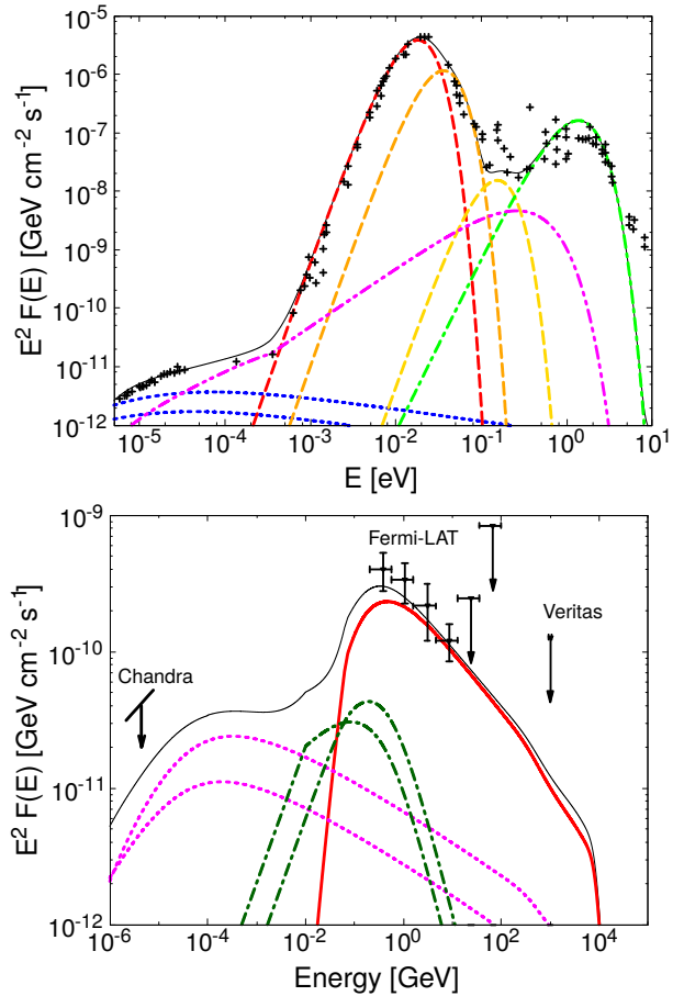
Figure 7. Multiwavelength spectrum of Arp220. The line style is the same of figure 5. Gamma-ray data are taken from Peng et al. (2016) , whereas the X-ray point (which again we take as upper limit for our diffuse flux taking into account possible contamination from pointlike sources and thermal plasma) has been taken from Paggi et al. (2017) .
