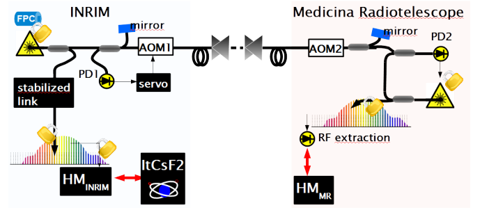
Fig. 2. The setup of our experiment. A fiber laser is frequency-locked to a high-finesse Fabry-Pérot cavity (FPC) and used as a transfer laser. Its frequency is measured against HM_{INRIM} using a fiber optical frequency comb; HM_{INRIM} is constantly measured by the primary frequency standard ItCsF2. The transfer laser is sent to Medicina Radiotelescope (MR) via a phase-stabilized optical link and here regenerated by phase-locking a diode laser to it. The regenerated radiation is used as a reference to stabilize an optical comb; the 40th harmonic of the repetition rate is extracted, divided by 100 and compared to HM_{MR} . AOM: acousto-optic modulators; PD: photodiodes; triangles represent bidirectional Erbium-Doped Fiber Amplifiers
