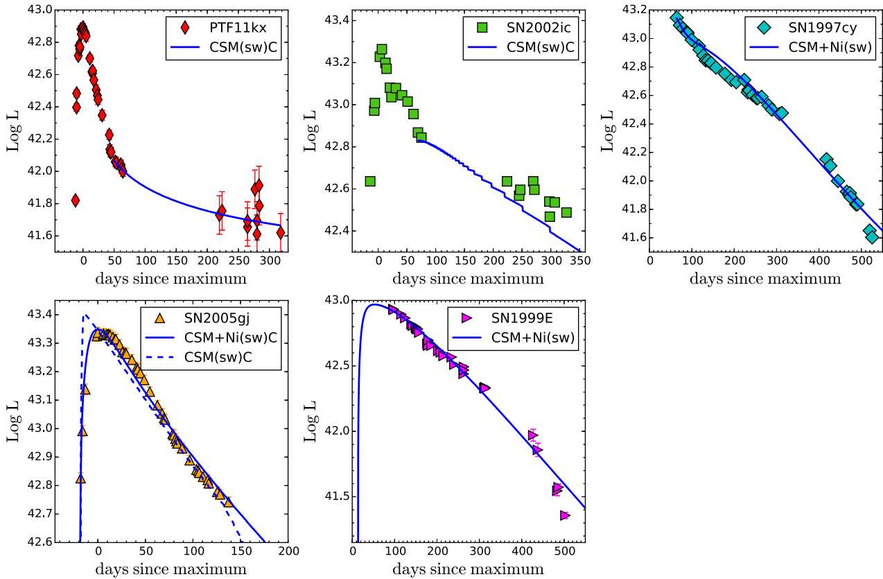
Figure 14. Pseudo-bolometric light curves of PTF11kx, SN 2002ic, SN 1997cy, SN 2005gj and SN 1999E and the semi-analytical model that best fit the light curve (blue solid line). The model used is reported in the legend. The suffix C refers to the model with constraints (see the text).
