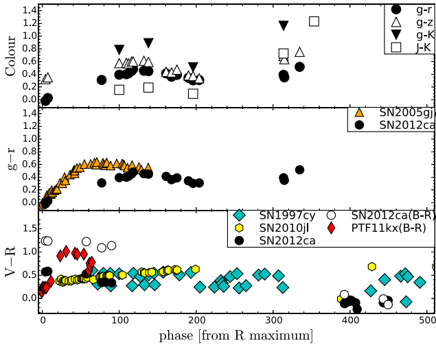
Figure 3. Top: dereddened colour evolutions of SN 2012ca. Middle: comparison of the dereddened g - r colour curves of SN 2012ca and SN 2005gj. Bottom: comparison of SN 2012ca dereddened V - R and B - R colour curves with that of PTF11kx ( B - R ) with those of SNe 1997cy and 2010jl (both V - R ).
