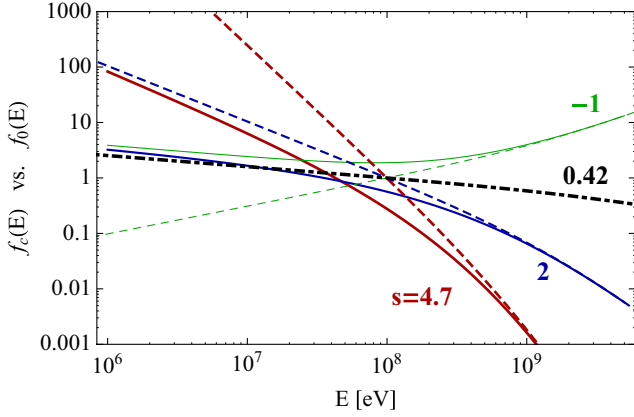
Figure 3. Spectra of cosmic rays inside a molecular cloud of column density N_H = 3 \times 10^{21} \text{ cm}^{-2} (solid lines) assuming that the spectra far from the cloud are given by power law in momentum of slope s (dashed lines). The dot-dashed line shows the eigenfunction of the problem.
